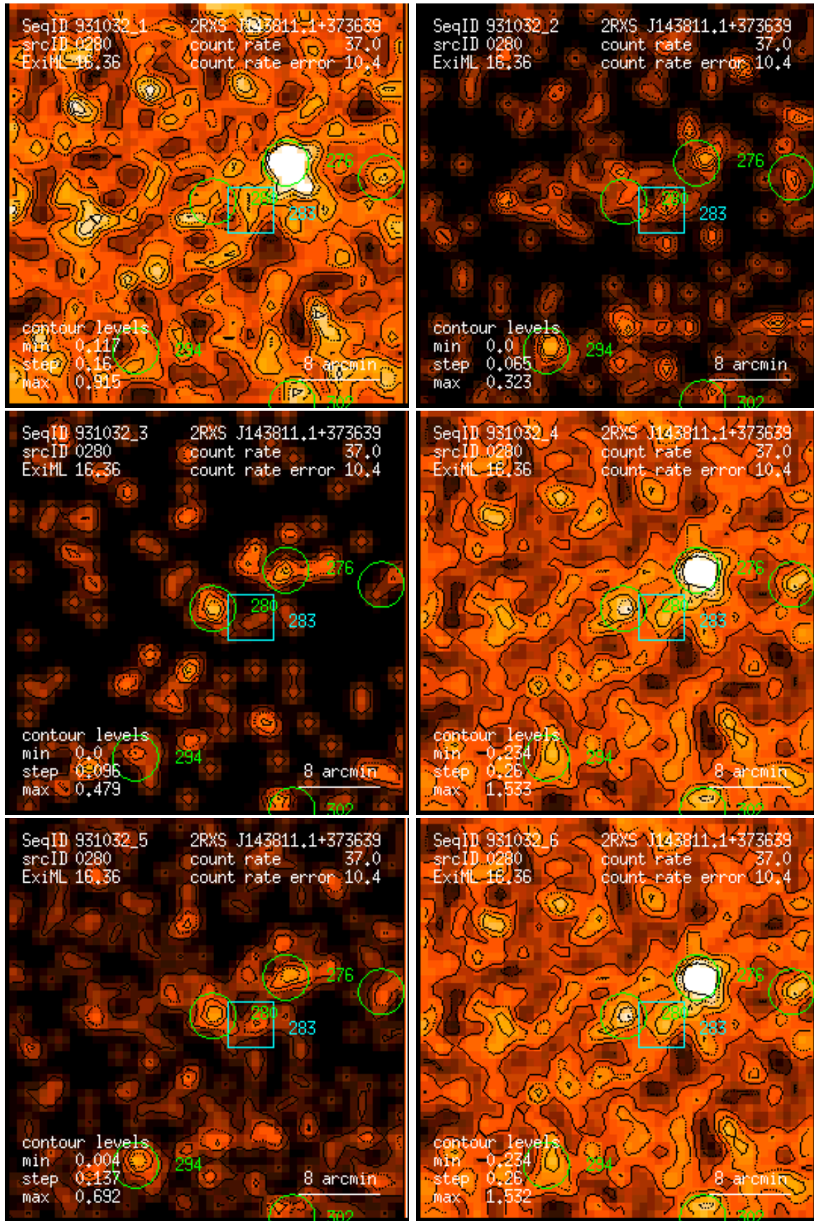
Figure 280: RASS 931032: detection 0280: band rate images, Gaussian filter: (1) PSPC channels 11 – 41, (2) 52 – 90, (3) 91 – 201, (4) 11 – 235, (5) 52 – 201, (6) 11 – 201. Broad band rates in counts/ks. Band rate contour levels in counts/ks/arcmin 2 .
