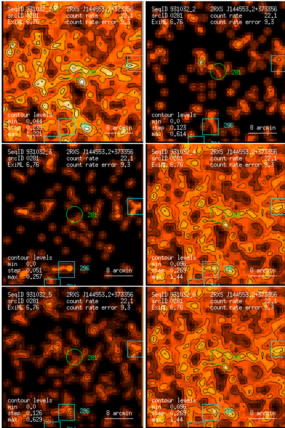
Figure 281: RASS 931032: detection 0281: band rate images, Gaussian filter: (1) PSPC channels 11 – 41, (2) 52 – 90, (3) 91 – 201, (4) 11 – 235, (5) 52 – 201, (6) 11 – 201. Broad band rates in counts/ks. Band rate contour levels in counts/ks/arcmin 2 .
