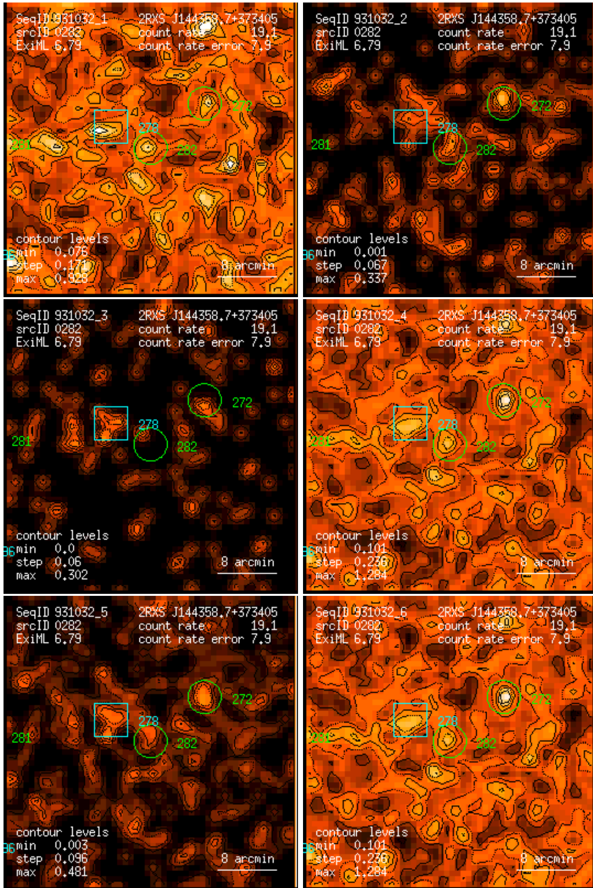
Figure 282: RASS 931032: detection 0282: band rate images, Gaussian filter: (1) PSPC channels 11 – 41, (2) 52 – 90, (3) 91 – 201, (4) 11 – 235, (5) 52 – 201, (6) 11 – 201. Broad band rates in counts/ks. Band rate contour levels in counts/ks/arcmin 2 .
