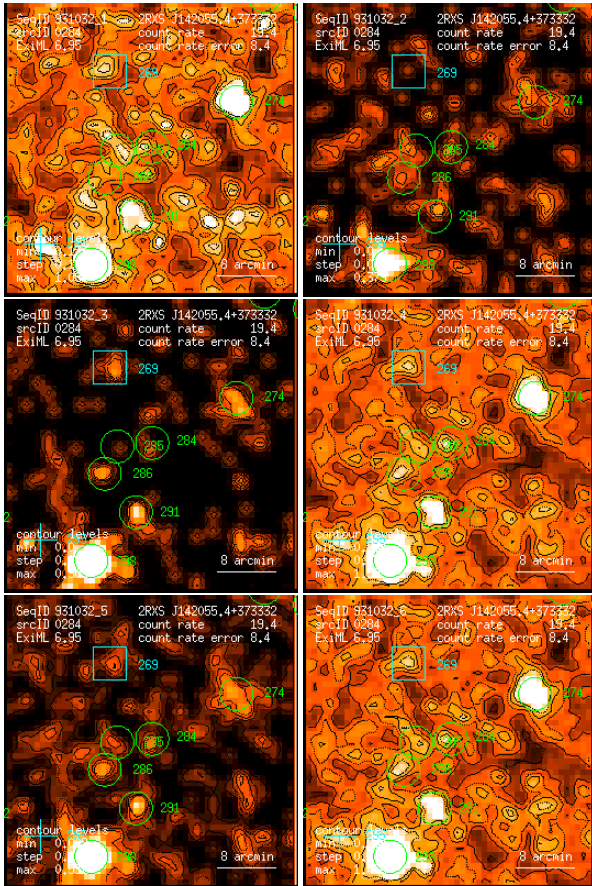
Figure 284: RASS 931032: detection 0284: band rate images, Gaussian filter: (1) PSPC channels 11 – 41, (2) 52 – 90, (3) 91 – 201, (4) 11 – 235, (5) 52 – 201, (6) 11 – 201. Broad band rates in counts/ks. Band rate contour levels in counts/ks/arcmin 2 .
