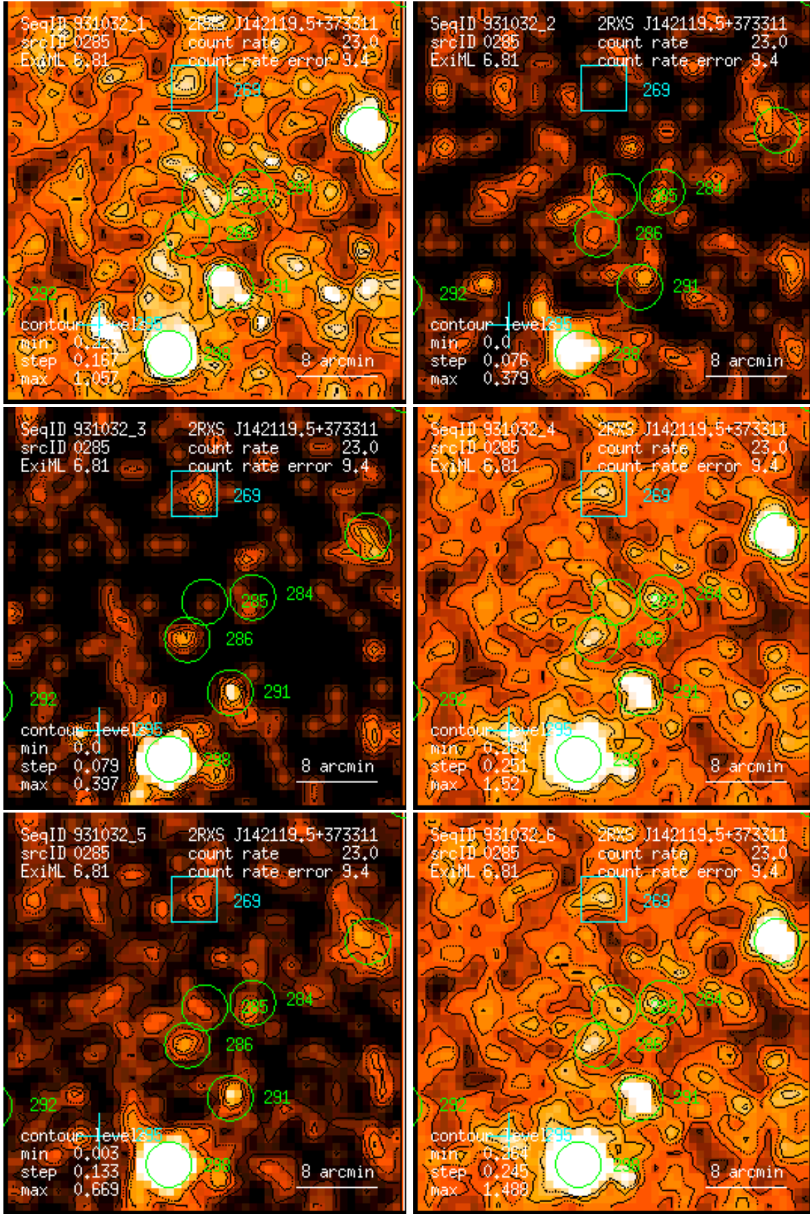
Figure 285: RASS 931032: detection 0285: band rate images, Gaussian filter: (1) PSPC channels 11 – 41, (2) 52 – 90, (3) 91 – 201, (4) 11 – 235, (5) 52 – 201, (6) 11 – 201. Broad band rates in counts/ks. Band rate contour levels in counts/ks/arcmin 2 .
