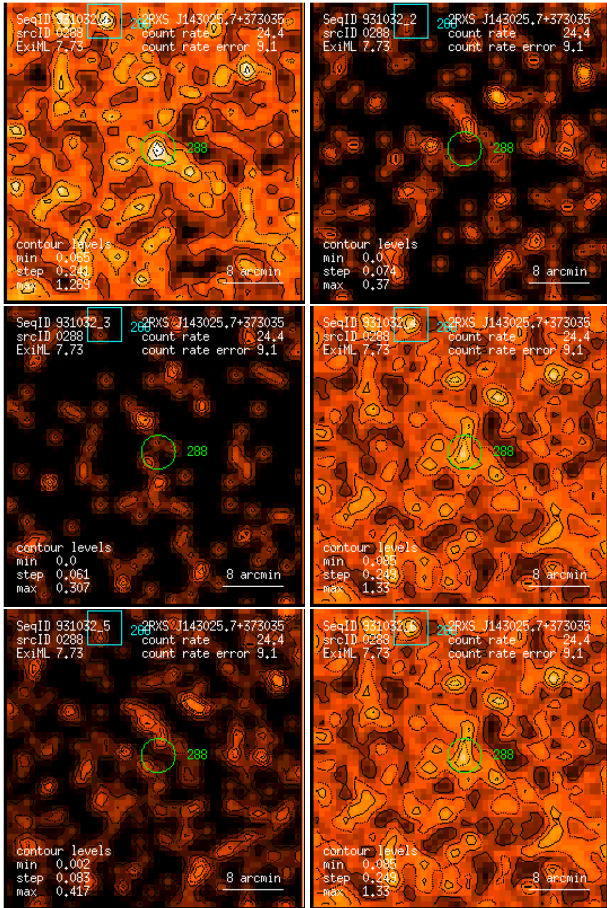
Figure 288: RASS 931032: detection 0288: band rate images, Gaussian filter: (1) PSPC channels 11 – 41, (2) 52 – 90, (3) 91 – 201, (4) 11 – 235, (5) 52 – 201, (6) 11 – 201. Broad band rates in counts/ks. Band rate contour levels in counts/ks/arcmin 2 .
