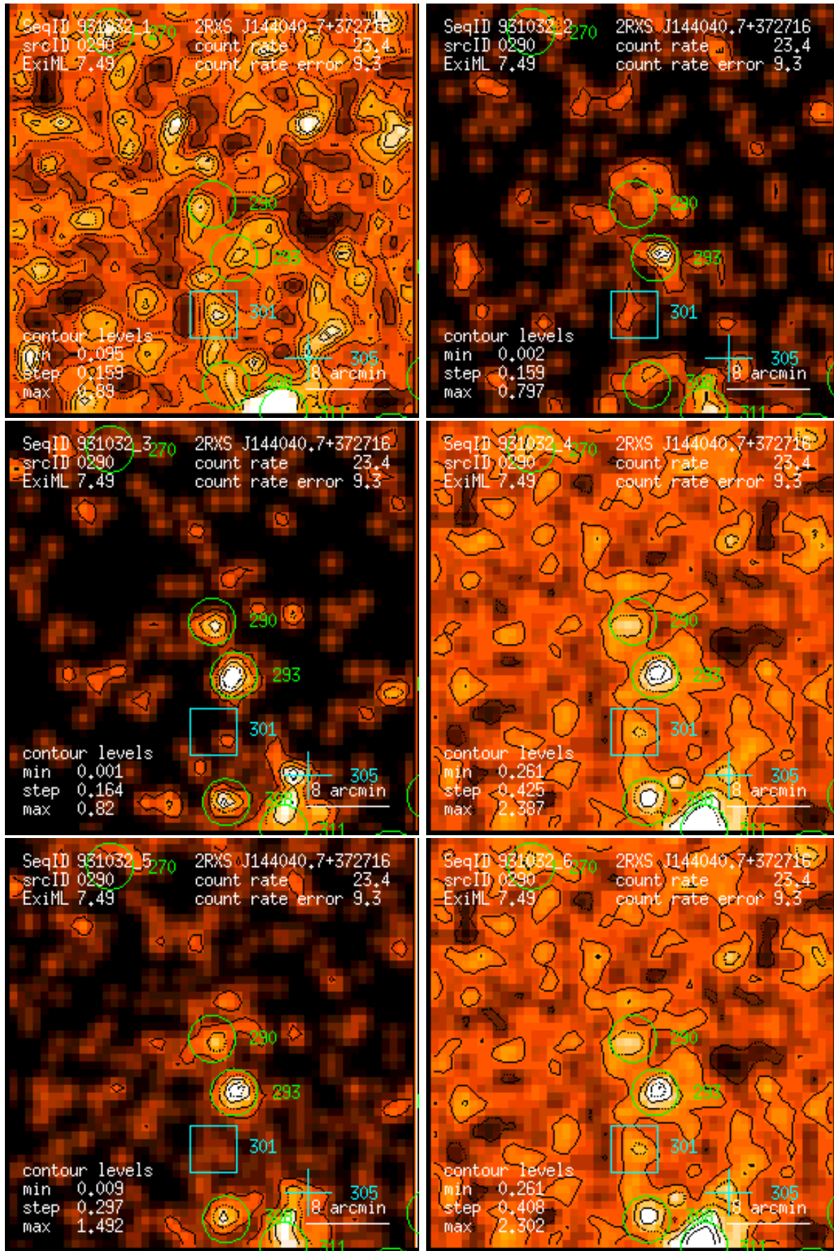
Figure 290: RASS 931032: detection 0290: band rate images, Gaussian filter: (1) PSPC channels 11 – 41, (2) 52 – 90, (3) 91 – 201, (4) 11 – 235, (5) 52 – 201, (6) 11 – 201. Broad band rates in counts/ks. Band rate contour levels in counts/ks/arcmin 2 .
