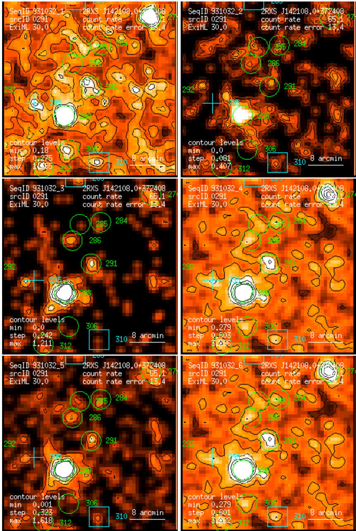
Figure 291: RASS 931032: detection 0291: band rate images, Gaussian filter: (1) PSPC channels 11 – 41, (2) 52 – 90, (3) 91 – 201, (4) 11 – 235, (5) 52 – 201, (6) 11 – 201. Broad band rates in counts/ks. Band rate contour levels in counts/ks/arcmin 2 .
