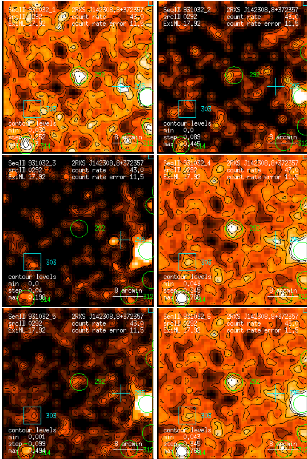
Figure 292: RASS 931032: detection 0292: band rate images, Gaussian filter: (1) PSPC channels 11 – 41, (2) 52 – 90, (3) 91 – 201, (4) 11 – 235, (5) 52 – 201, (6) 11 – 201. Broad band rates in counts/ks. Band rate contour levels in counts/ks/arcmin 2 .
