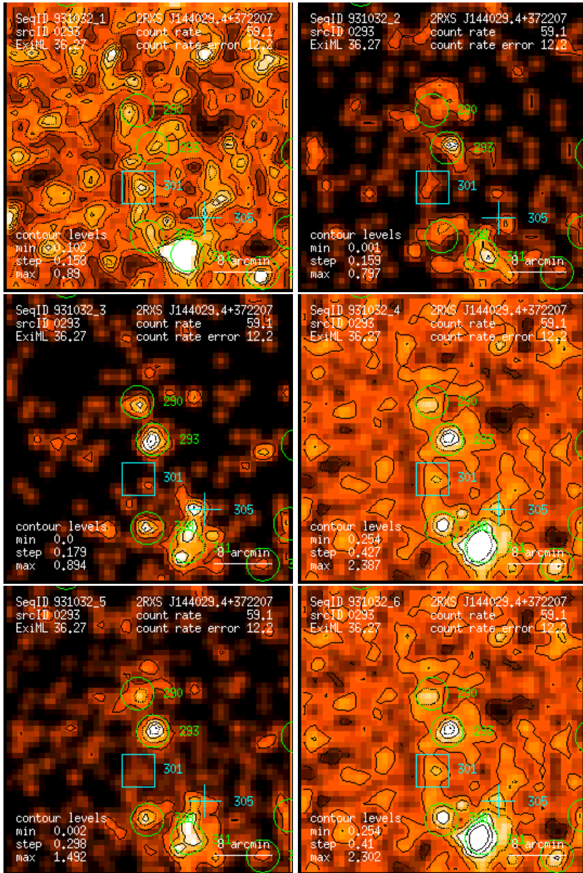
Figure 293: RASS 931032: detection 0293: band rate images, Gaussian filter: (1) PSPC channels 11 – 41, (2) 52 – 90, (3) 91 – 201, (4) 11 – 235, (5) 52 – 201, (6) 11 – 201. Broad band rates in counts/ks. Band rate contour levels in counts/ks/arcmin 2 .
