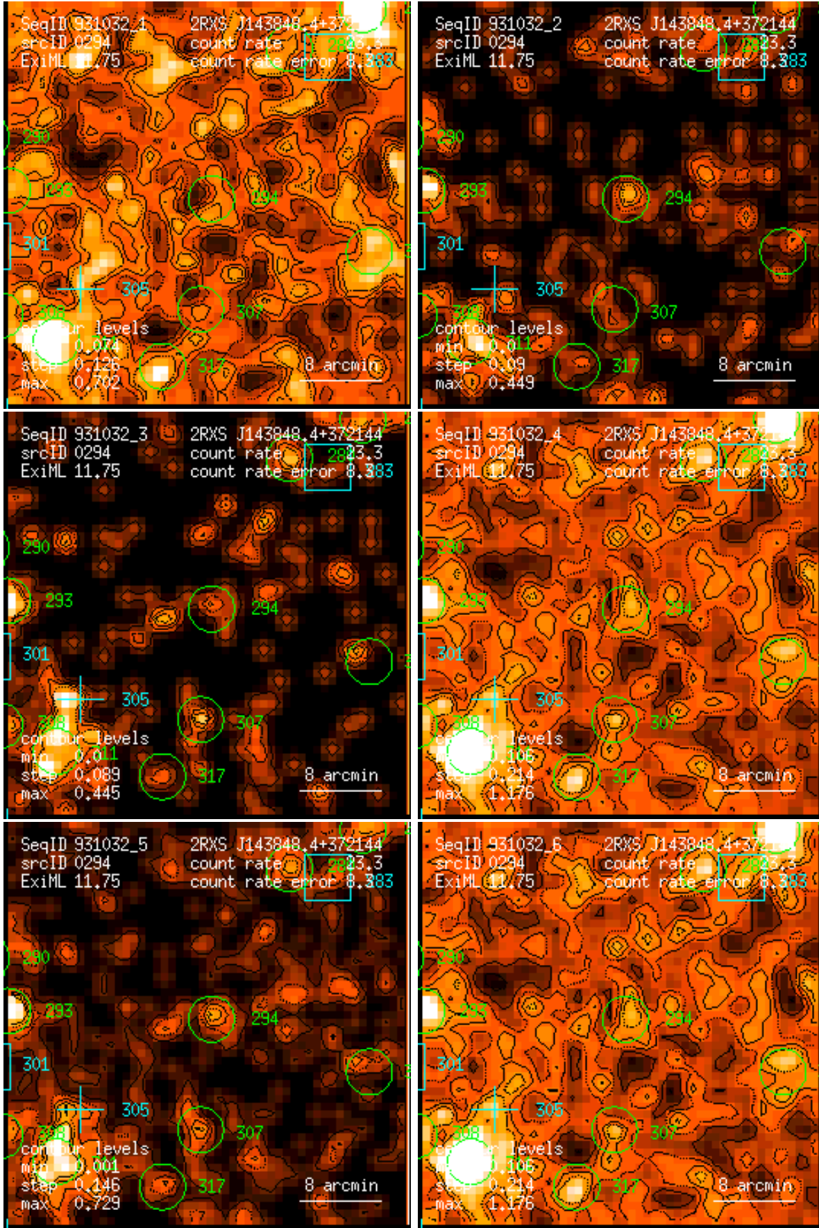
Figure 294: RASS 931032: detection 0294: band rate images, Gaussian filter: (1) PSPC channels 11 – 41, (2) 52 – 90, (3) 91 – 201, (4) 11 – 235, (5) 52 – 201, (6) 11 – 201. Broad band rates in counts/ks. Band rate contour levels in counts/ks/arcmin 2 .
