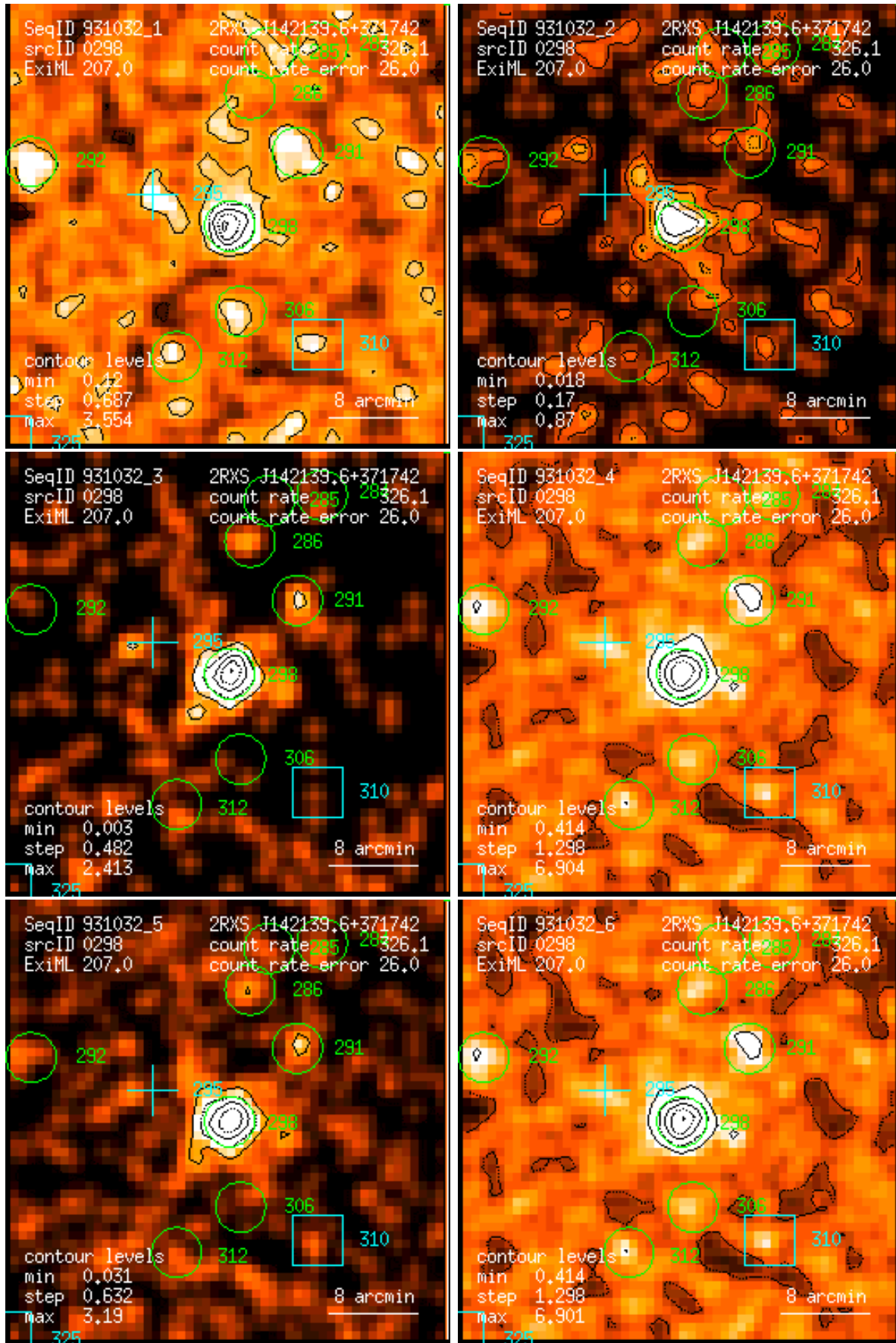
Figure 298: RASS 931032: detection 0298: band rate images, Gaussian filter: (1) PSPC channels 11 – 41, (2) 52 – 90, (3) 91 – 201, (4) 11 – 235, (5) 52 – 201, (6) 11 – 201. Broad band rates in counts/ks. Band rate contour levels in counts/ks/arcmin 2 .
