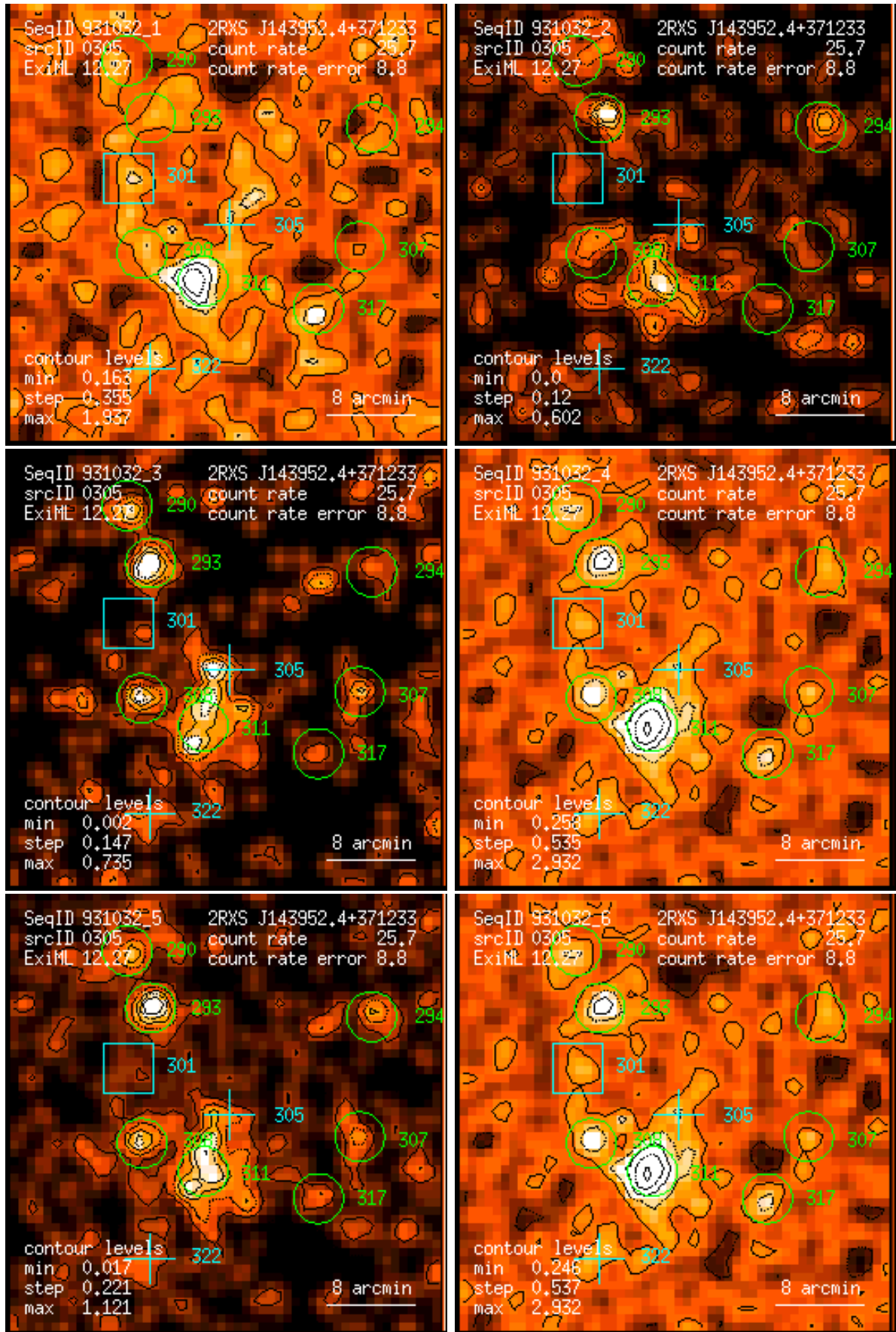
Figure 305: RASS 931032: detection 0305: band rate images, Gaussian filter: (1) PSPC channels 11 – 41, (2) 52 – 90, (3) 91 – 201, (4) 11 – 235, (5) 52 – 201, (6) 11 – 201. Broad band rates in counts/ks. Band rate contour levels in counts/ks/arcmin 2 .
