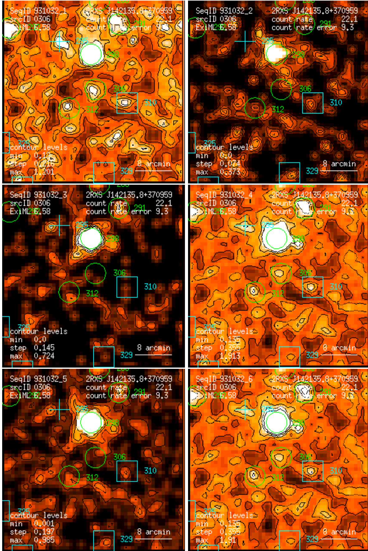
Figure 306: RASS 931032: detection 0306: band rate images, Gaussian filter: (1) PSPC channels 11 – 41, (2) 52 – 90, (3) 91 – 201, (4) 11 – 235, (5) 52 – 201, (6) 11 – 201. Broad band rates in counts/ks. Band rate contour levels in counts/ks/arcmin 2 .
