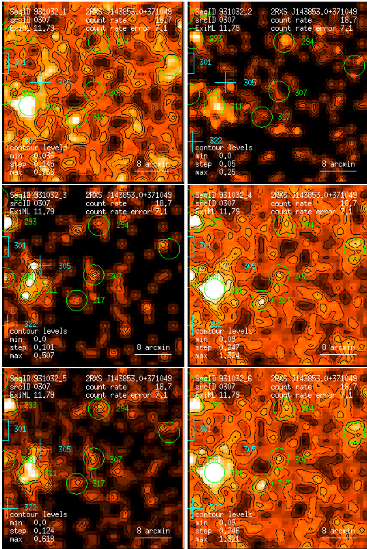
Figure 307: RASS 931032: detection 0307: band rate images, Gaussian filter: (1) PSPC channels 11 – 41, (2) 52 – 90, (3) 91 – 201, (4) 11 – 235, (5) 52 – 201, (6) 11 – 201. Broad band rates in counts/ks. Band rate contour levels in counts/ks/arcmin 2 .
