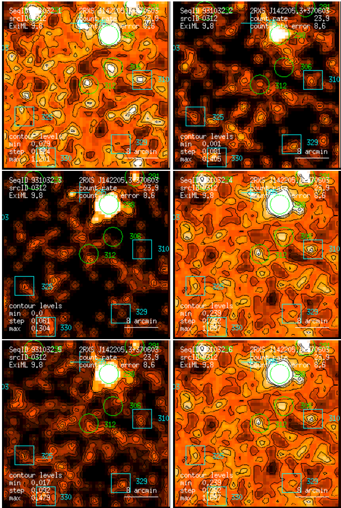
Figure 312: RASS 931032: detection 0312: band rate images, Gaussian filter: (1) PSPC channels 11 – 41, (2) 52 – 90, (3) 91 – 201, (4) 11 – 235, (5) 52 – 201, (6) 11 – 201. Broad band rates in counts/ks. Band rate contour levels in counts/ks/arcmin 2 .
