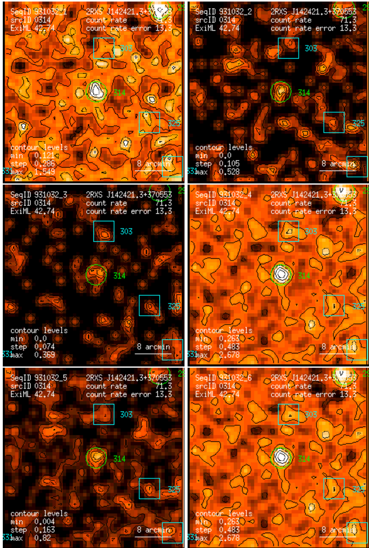
Figure 314: RASS 931032: detection 0314: band rate images, Gaussian filter: (1) PSPC channels 11 – 41, (2) 52 – 90, (3) 91 – 201, (4) 11 – 235, (5) 52 – 201, (6) 11 – 201. Broad band rates in counts/ks. Band rate contour levels in counts/ks/arcmin 2 .
