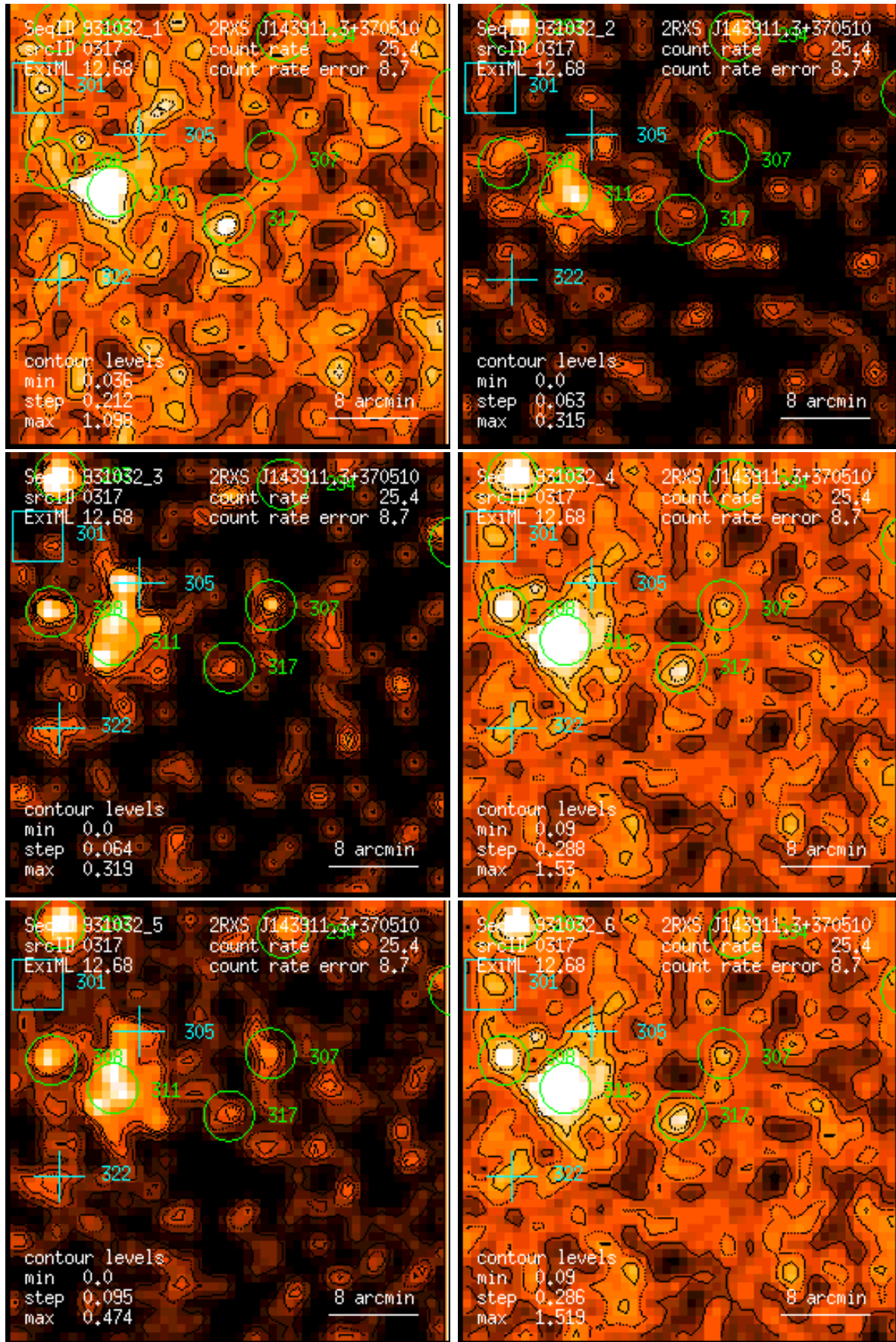
Figure 317: RASS 931032: detection 0317: band rate images, Gaussian filter: (1) PSPC channels 11 – 41, (2) 52 – 90, (3) 91 – 201, (4) 11 – 235, (5) 52 – 201, (6) 11 – 201. Broad band rates in counts/ks. Band rate contour levels in counts/ks/arcmin 2 .
