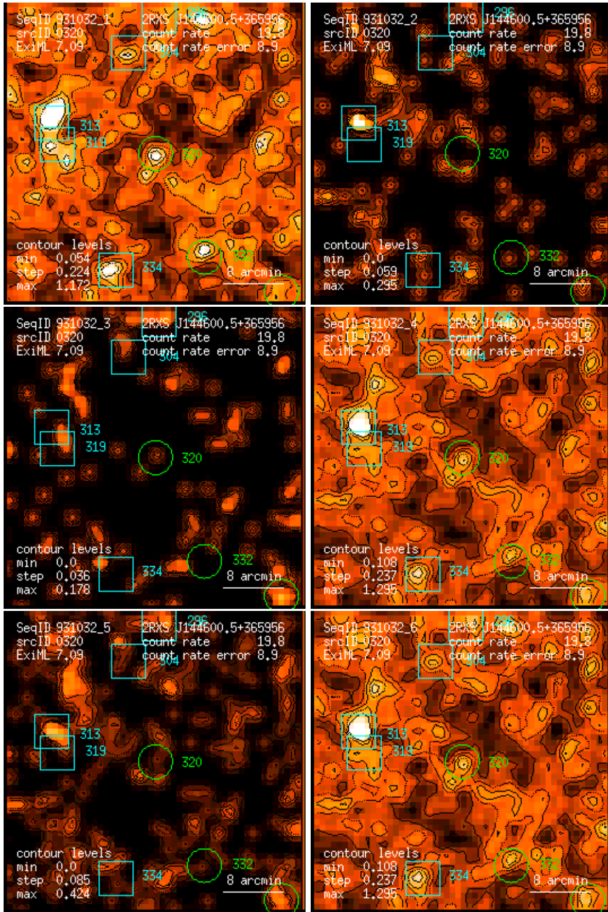
Figure 320: RASS 931032: detection 0320: band rate images, Gaussian filter: (1) PSPC channels 11 – 41, (2) 52 – 90, (3) 91 – 201, (4) 11 – 235, (5) 52 – 201, (6) 11 – 201. Broad band rates in counts/ks. Band rate contour levels in counts/ks/arcmin 2 .
