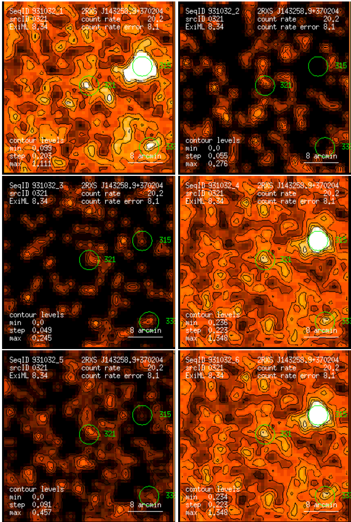
Figure 321: RASS 931032: detection 0321: band rate images, Gaussian filter: (1) PSPC channels 11 – 41, (2) 52 – 90, (3) 91 – 201, (4) 11 – 235, (5) 52 – 201, (6) 11 – 201. Broad band rates in counts/ks. Band rate contour levels in counts/ks/arcmin 2 .
