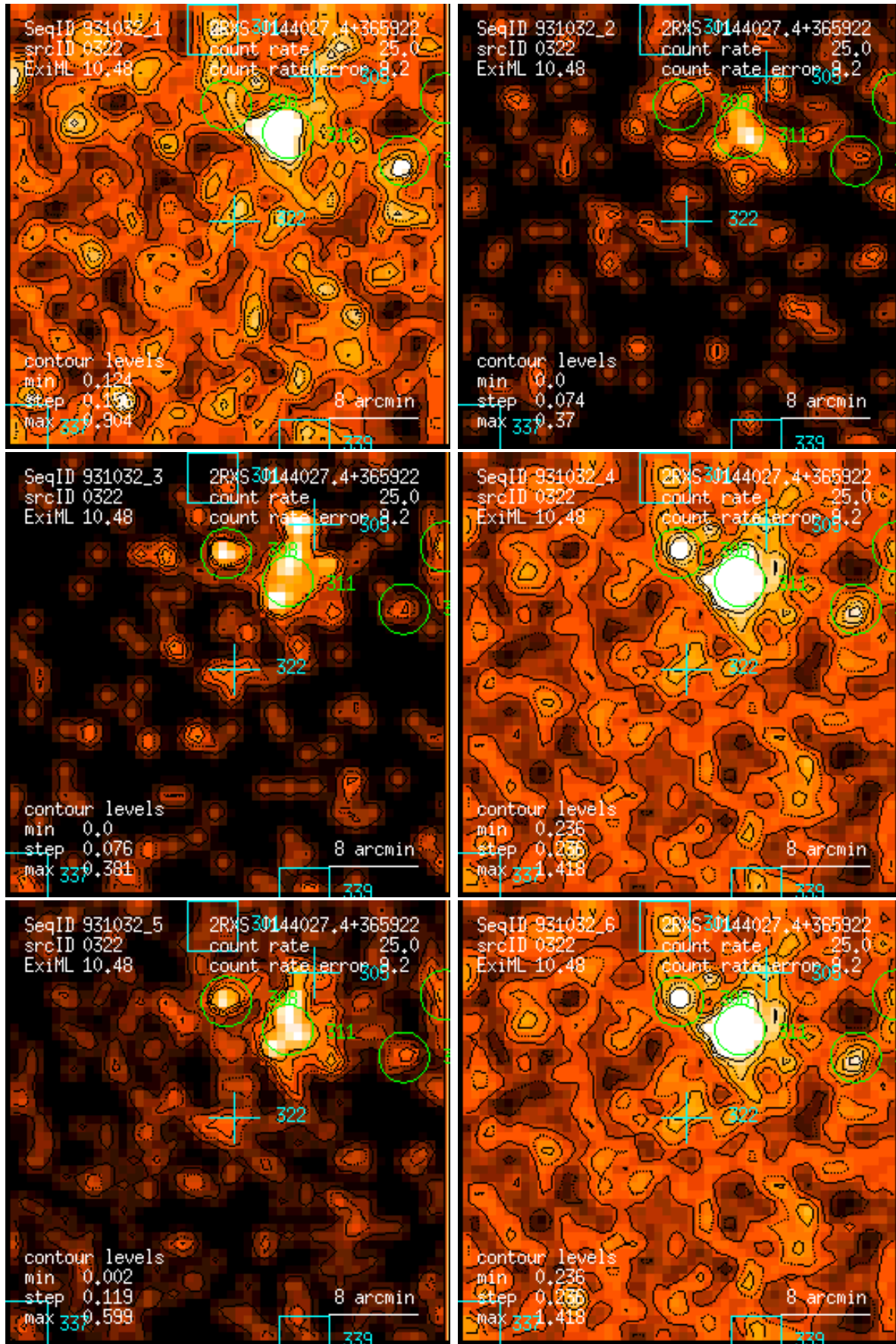
Figure 322: RASS 931032: detection 0322: band rate images, Gaussian filter: (1) PSPC channels 11 – 41, (2) 52 – 90, (3) 91 – 201, (4) 11 – 235, (5) 52 – 201, (6) 11 – 201. Broad band rates in counts/ks. Band rate contour levels in counts/ks/arcmin 2 .
