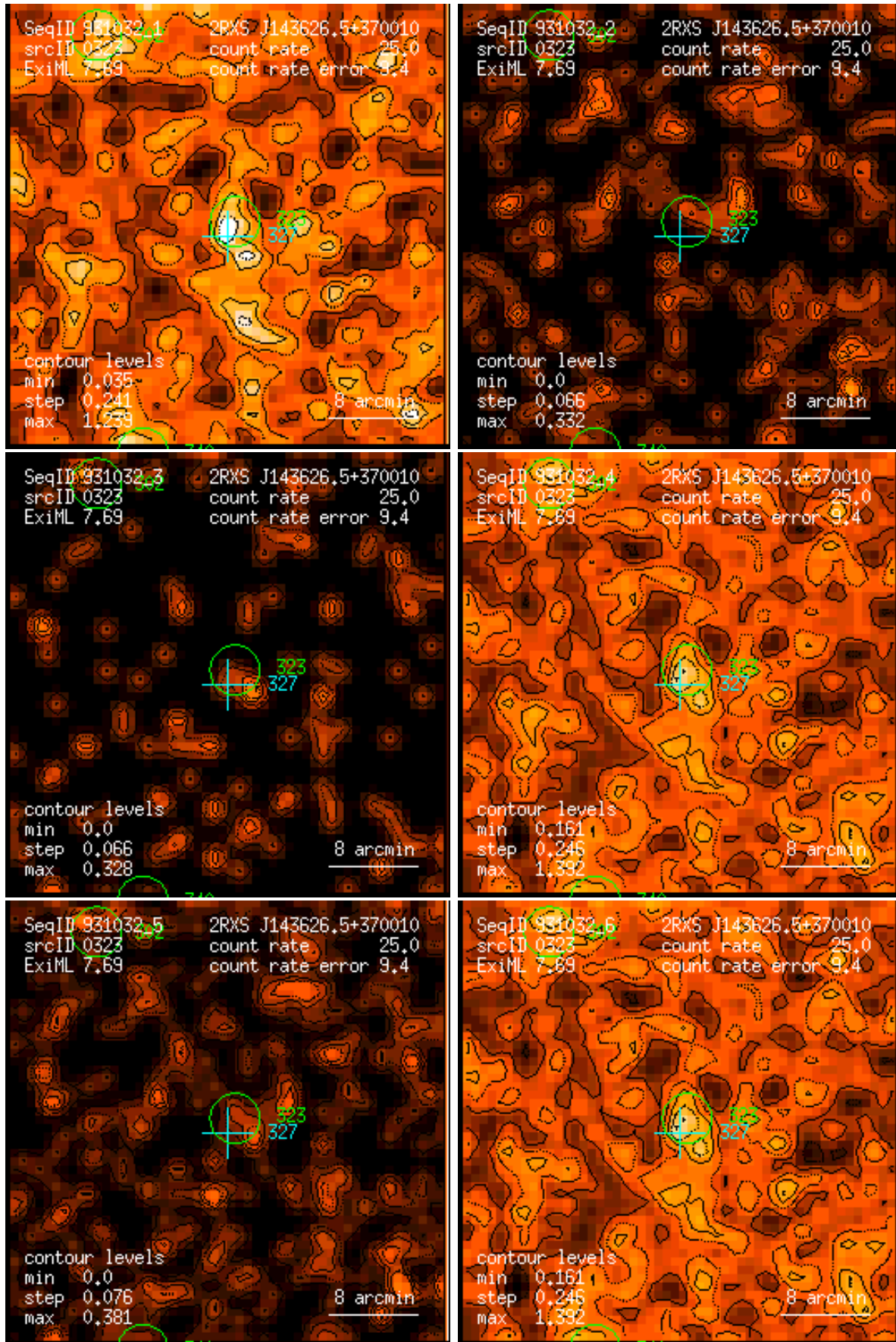
Figure 323: RASS 931032: detection 0323: band rate images, Gaussian filter: (1) PSPC channels 11 – 41, (2) 52 – 90, (3) 91 – 201, (4) 11 – 235, (5) 52 – 201, (6) 11 – 201. Broad band rates in counts/ks. Band rate contour levels in counts/ks/arcmin 2 .
