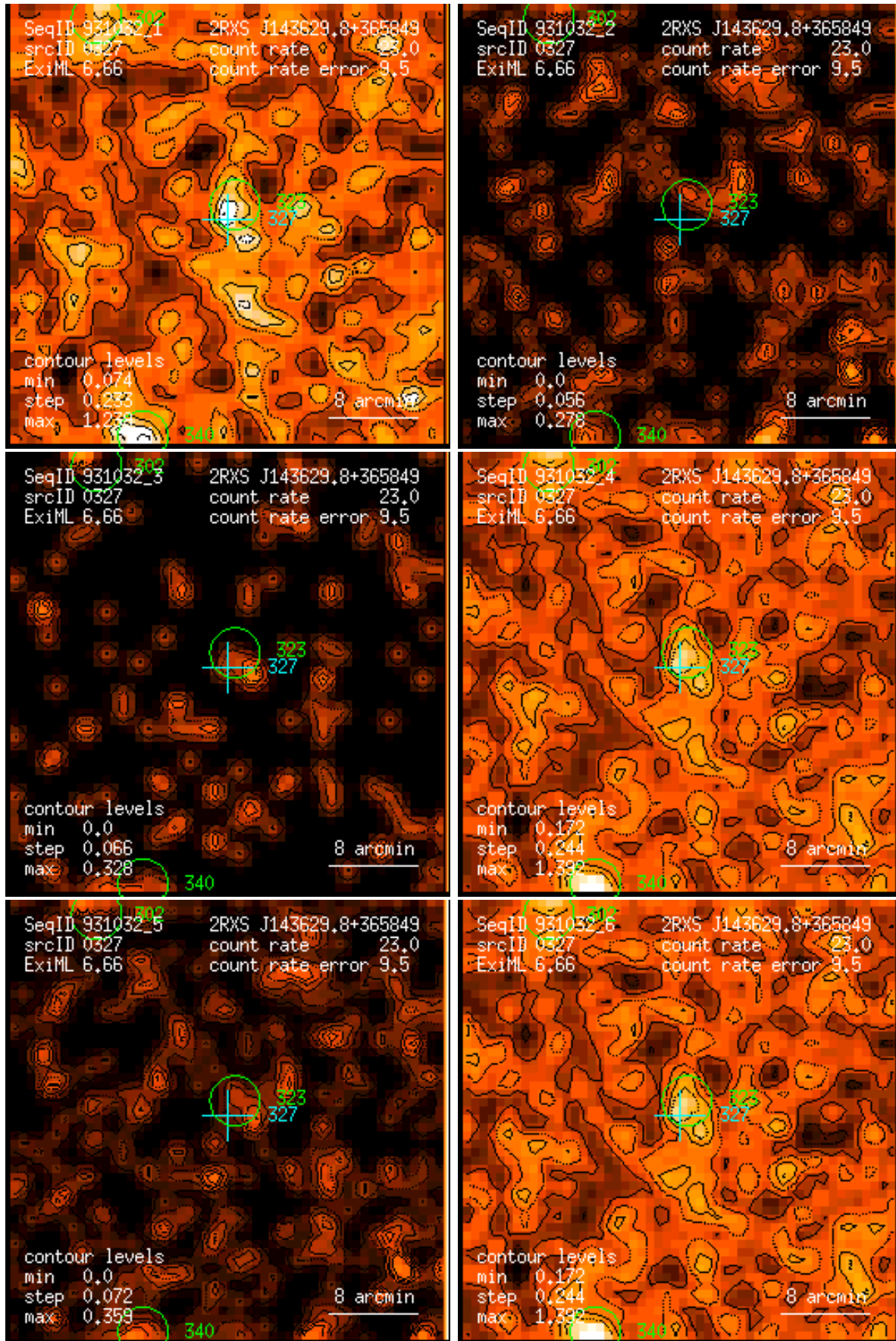
Figure 327: RASS 931032: detection 0327: band rate images, Gaussian filter: (1) PSPC channels 11 – 41, (2) 52 – 90, (3) 91 – 201, (4) 11 – 235, (5) 52 – 201, (6) 11 – 201. Broad band rates in counts/ks. Band rate contour levels in counts/ks/arcmin 2 .
