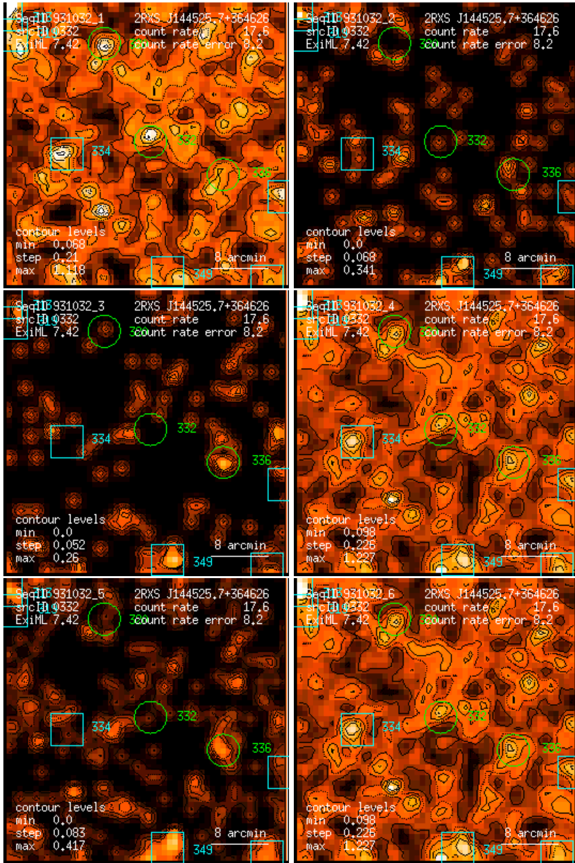
Figure 332: RASS 931032: detection 0332: band rate images, Gaussian filter: (1) PSPC channels 11 – 41, (2) 52 – 90, (3) 91 – 201, (4) 11 – 235, (5) 52 – 201, (6) 11 – 201. Broad band rates in counts/ks. Band rate contour levels in counts/ks/arcmin 2 .
