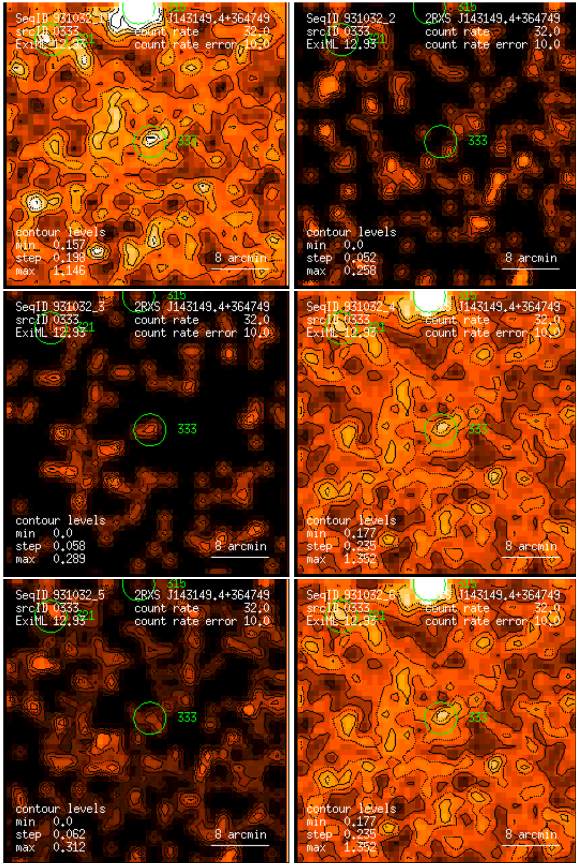
Figure 333: RASS 931032: detection 0333: band rate images, Gaussian filter: (1) PSPC channels 11 – 41, (2) 52 – 90, (3) 91 – 201, (4) 11 – 235, (5) 52 – 201, (6) 11 – 201. Broad band rates in counts/ks. Band rate contour levels in counts/ks/arcmin 2 .
