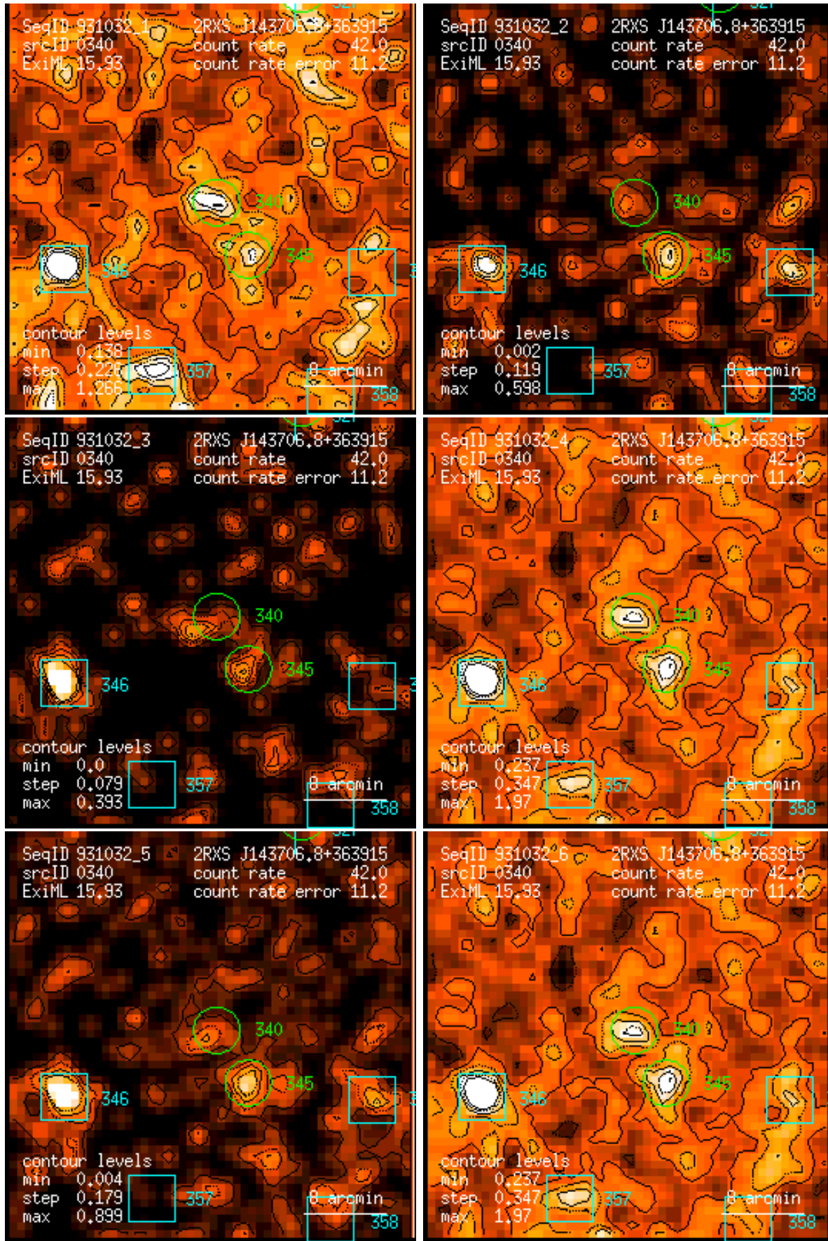
Figure 340: RASS 931032: detection 0340: band rate images, Gaussian filter: (1) PSPC channels 11 – 41, (2) 52 – 90, (3) 91 – 201, (4) 11 – 235, (5) 52 – 201, (6) 11 – 201. Broad band rates in counts/ks. Band rate contour levels in counts/ks/arcmin 2 .
