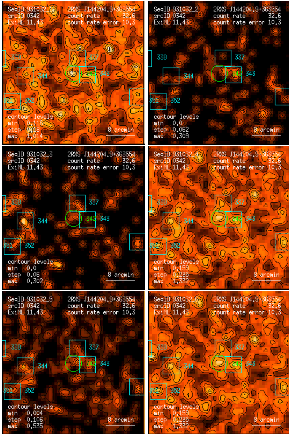
Figure 342: RASS 931032: detection 0342: band rate images, Gaussian filter: (1) PSPC channels 11 – 41, (2) 52 – 90, (3) 91 – 201, (4) 11 – 235, (5) 52 – 201, (6) 11 – 201. Broad band rates in counts/ks. Band rate contour levels in counts/ks/arcmin 2 .
