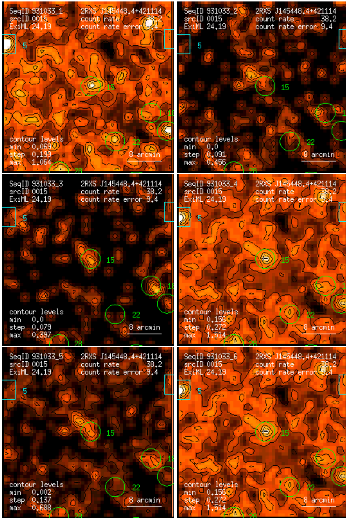
Figure 15: RASS 931033: detection 0015: band rate images, Gaussian filter: (1) PSPC channels 11 – 41, (2) 52 – 90, (3) 91 – 201, (4) 11 – 235, (5) 52 – 201, (6) 11 – 201. Broad band rates in counts/ks. Band rate contour levels in counts/ks/arcmin 2 .
