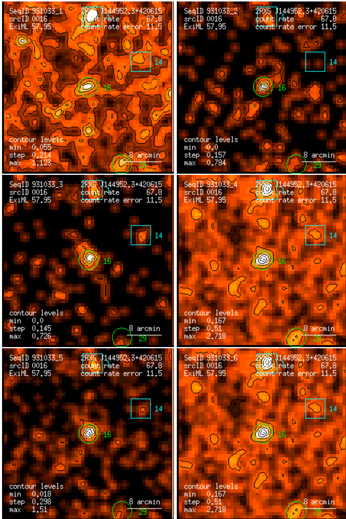
Figure 16: RASS 931033: detection 0016: band rate images, Gaussian filter: (1) PSPC channels 11 – 41, (2) 52 – 90, (3) 91 – 201, (4) 11 – 235, (5) 52 – 201, (6) 11 – 201. Broad band rates in counts/ks. Band rate contour levels in counts/ks/arcmin 2 .
