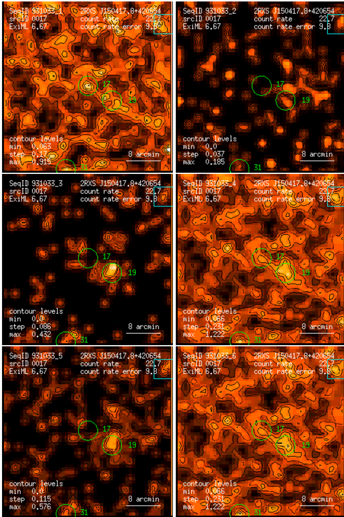
Figure 17: RASS 931033: detection 0017: band rate images, Gaussian filter: (1) PSPC channels 11 – 41, (2) 52 – 90, (3) 91 – 201, (4) 11 – 235, (5) 52 – 201, (6) 11 – 201. Broad band rates in counts/ks. Band rate contour levels in counts/ks/arcmin 2 .
