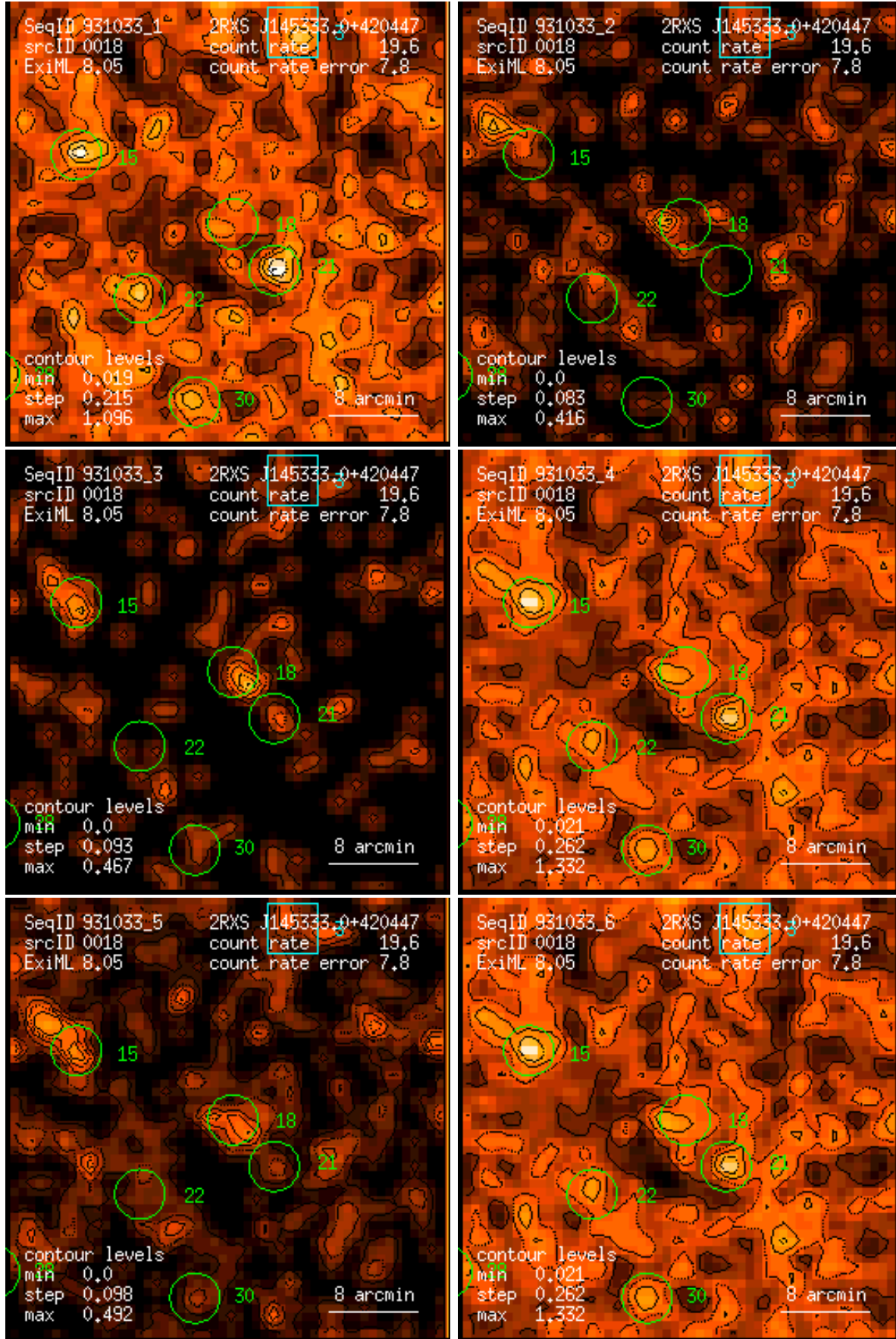
Figure 18: RASS 931033: detection 0018: band rate images, Gaussian filter: (1) PSPC channels 11 – 41, (2) 52 – 90, (3) 91 – 201, (4) 11 – 235, (5) 52 – 201, (6) 11 – 201. Broad band rates in counts/ks. Band rate contour levels in counts/ks/arcmin 2 .
