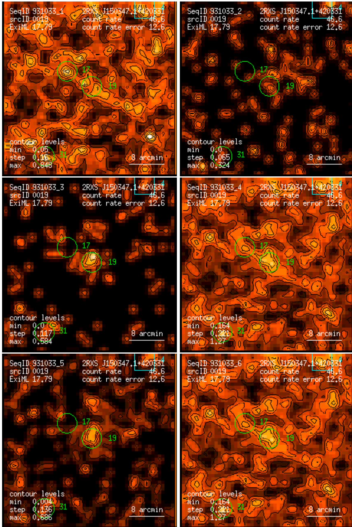
Figure 19: RASS 931033: detection 0019: band rate images, Gaussian filter: (1) PSPC channels 11 – 41, (2) 52 – 90, (3) 91 – 201, (4) 11 – 235, (5) 52 – 201, (6) 11 – 201. Broad band rates in counts/ks. Band rate contour levels in counts/ks/arcmin 2 .
