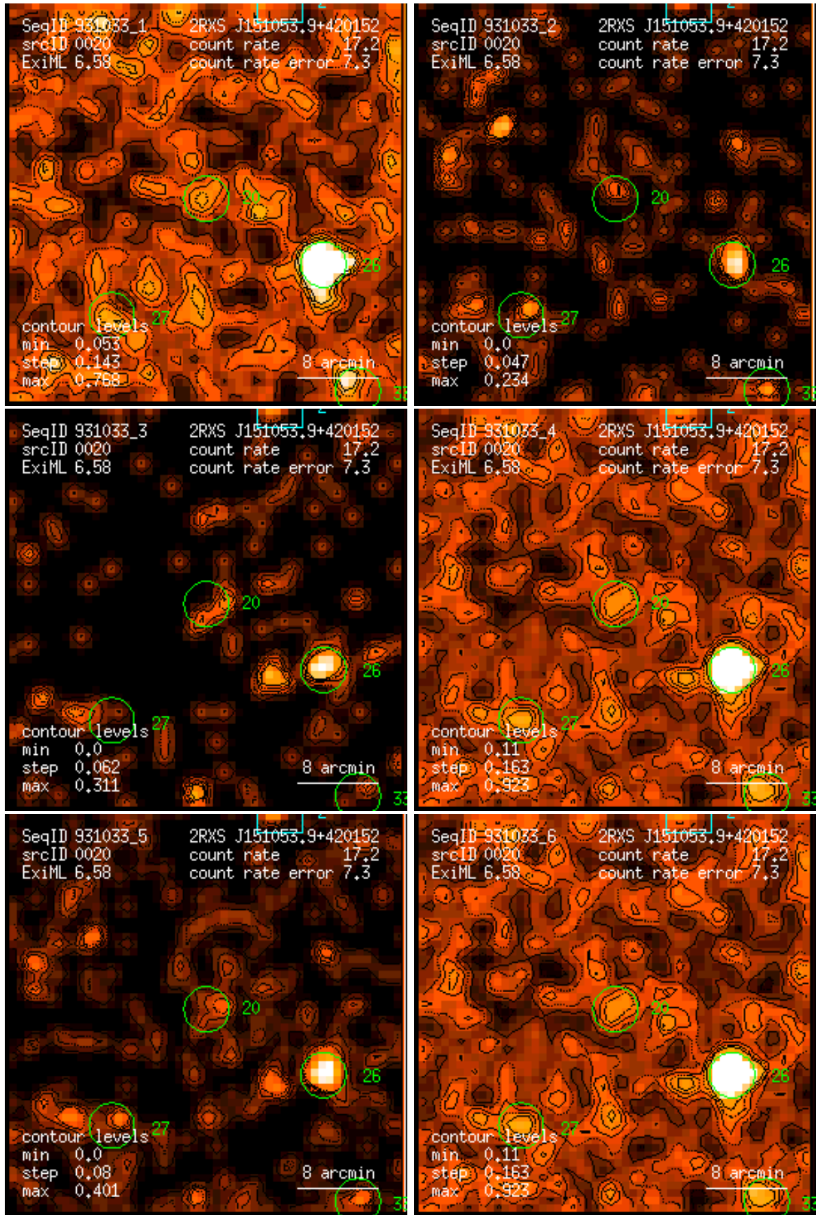
Figure 20: RASS 931033: detection 0020: band rate images, Gaussian filter: (1) PSPC channels 11 – 41, (2) 52 – 90, (3) 91 – 201, (4) 11 – 235, (5) 52 – 201, (6) 11 – 201. Broad band rates in counts/ks. Band rate contour levels in counts/ks/arcmin 2 .
