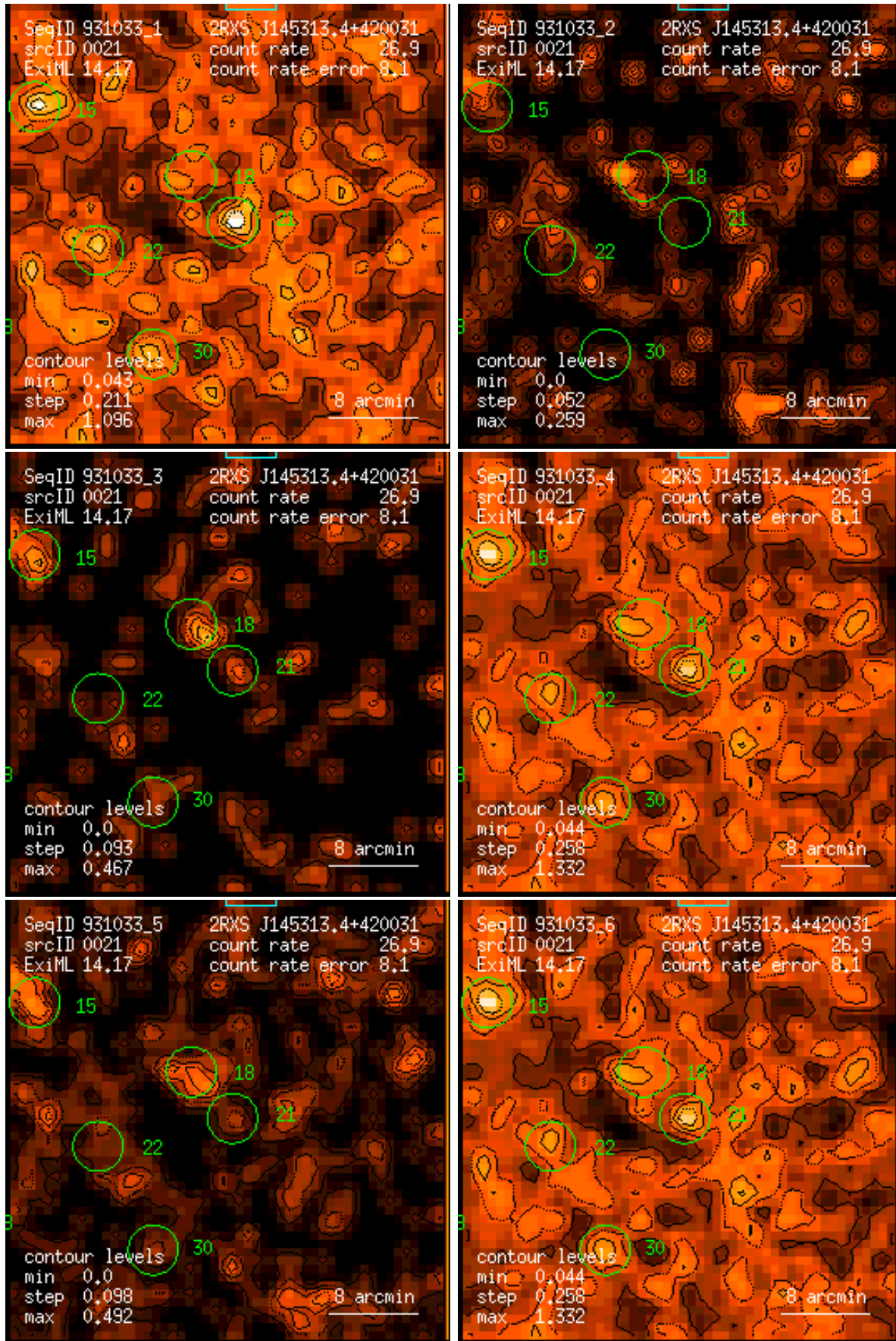
Figure 21: RASS 931033: detection 0021: band rate images, Gaussian filter: (1) PSPC channels 11 – 41, (2) 52 – 90, (3) 91 – 201, (4) 11 – 235, (5) 52 – 201, (6) 11 – 201. Broad band rates in counts/ks. Band rate contour levels in counts/ks/arcmin 2 .
