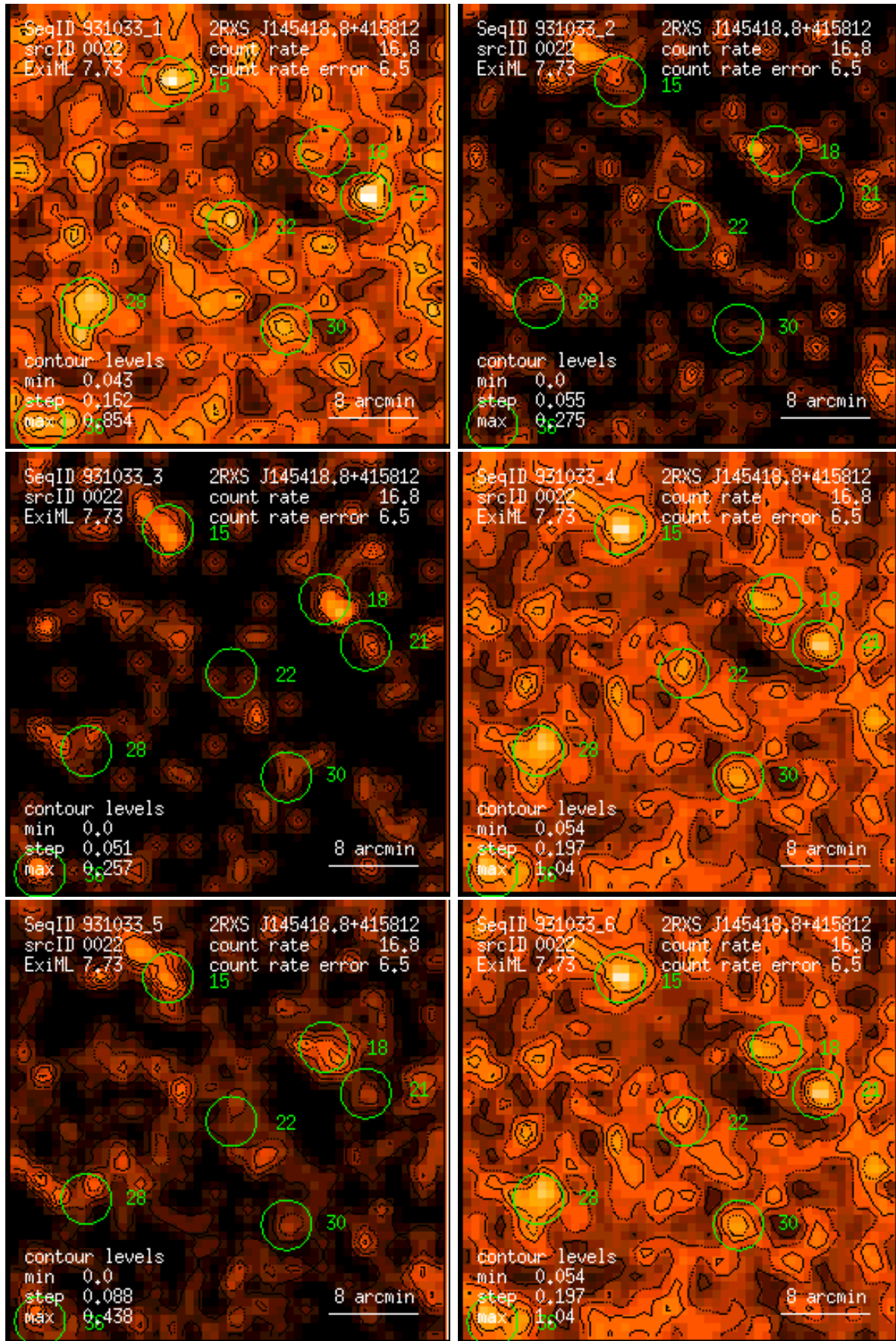
Figure 22: RASS 931033: detection 0022: band rate images, Gaussian filter: (1) PSPC channels 11 – 41, (2) 52 – 90, (3) 91 – 201, (4) 11 – 235, (5) 52 – 201, (6) 11 – 201. Broad band rates in counts/ks. Band rate contour levels in counts/ks/arcmin 2 .
