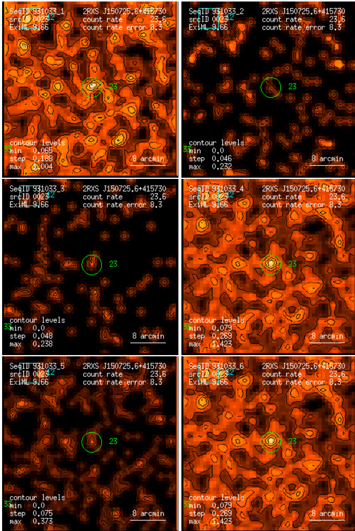
Figure 23: RASS 931033: detection 0023: band rate images, Gaussian filter: (1) PSPC channels 11 – 41, (2) 52 – 90, (3) 91 – 201, (4) 11 – 235, (5) 52 – 201, (6) 11 – 201. Broad band rates in counts/ks. Band rate contour levels in counts/ks/arcmin 2 .
