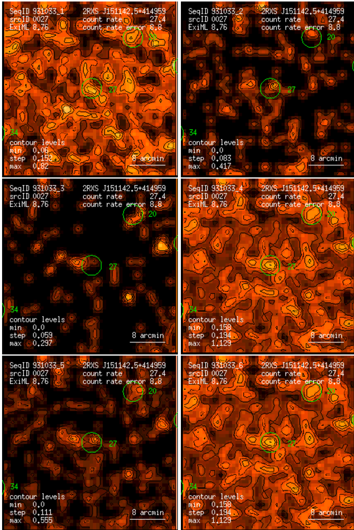
Figure 27: RASS 931033: detection 0027: band rate images, Gaussian filter: (1) PSPC channels 11 – 41, (2) 52 – 90, (3) 91 – 201, (4) 11 – 235, (5) 52 – 201, (6) 11 – 201. Broad band rates in counts/ks. Band rate contour levels in counts/ks/arcmin 2 .
