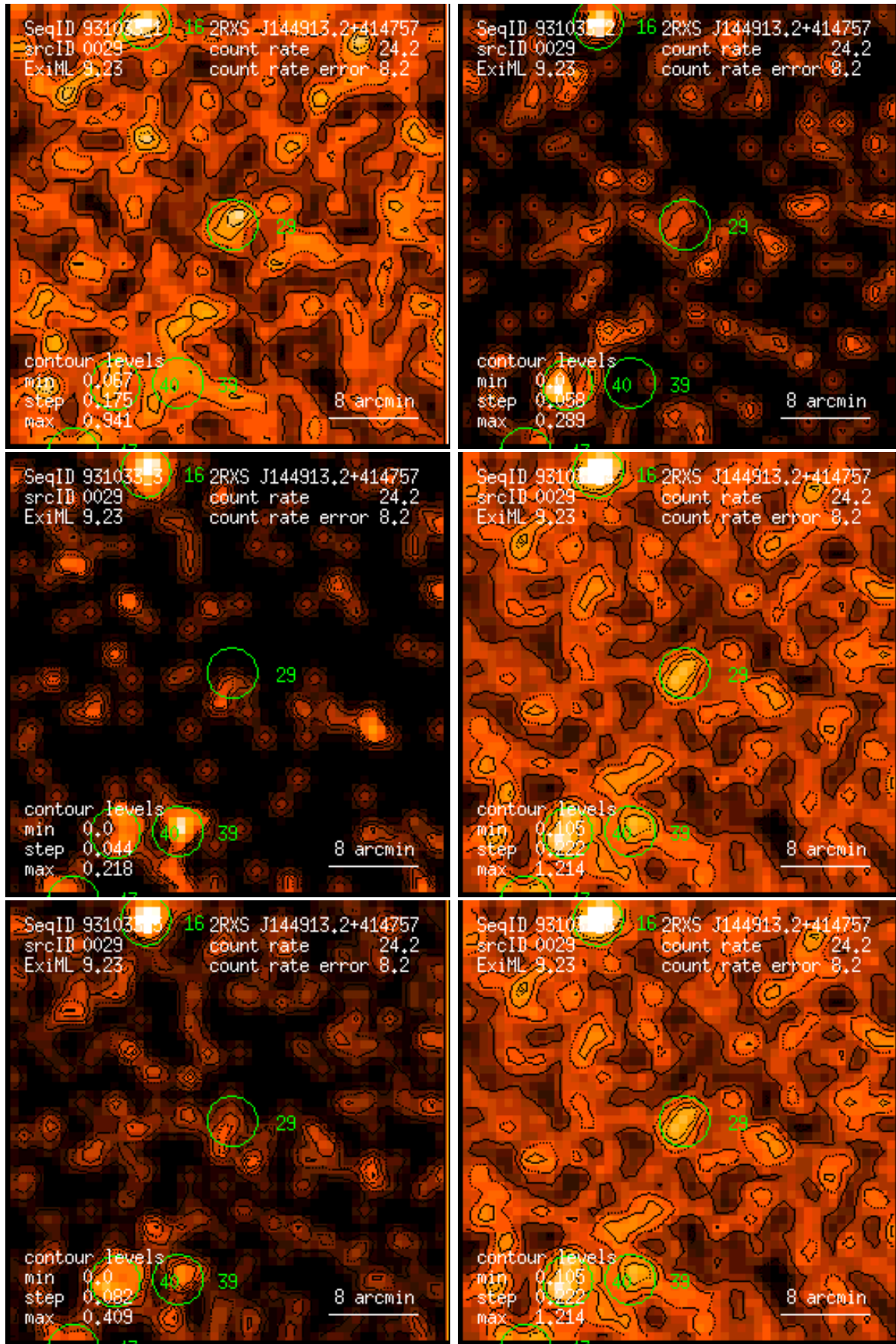
Figure 29: RASS 931033: detection 0029: band rate images, Gaussian filter: (1) PSPC channels 11 – 41, (2) 52 – 90, (3) 91 – 201, (4) 11 – 235, (5) 52 – 201, (6) 11 – 201. Broad band rates in counts/ks. Band rate contour levels in counts/ks/arcmin 2 .
