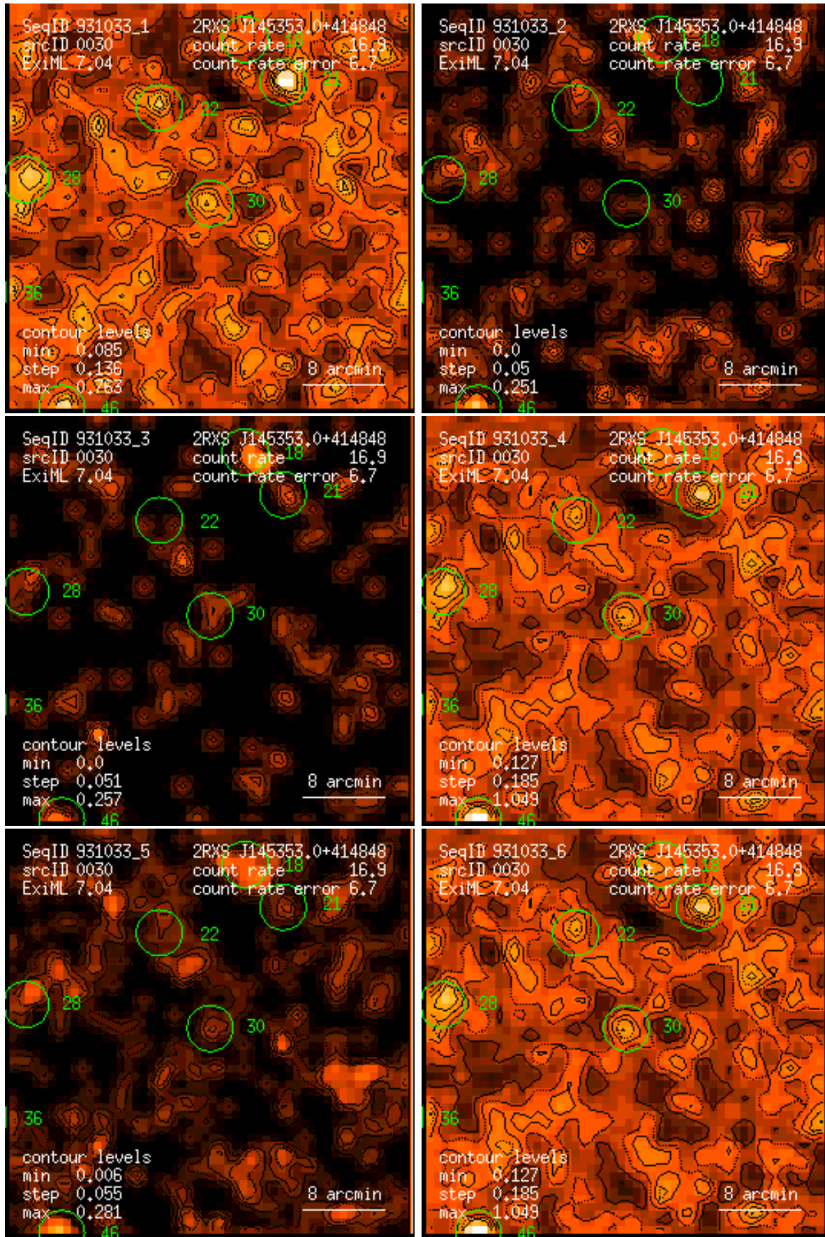
Figure 30: RASS 931033: detection 0030: band rate images, Gaussian filter: (1) PSPC channels 11 – 41, (2) 52 – 90, (3) 91 – 201, (4) 11 – 235, (5) 52 – 201, (6) 11 – 201. Broad band rates in counts/ks. Band rate contour levels in counts/ks/arcmin 2 .
