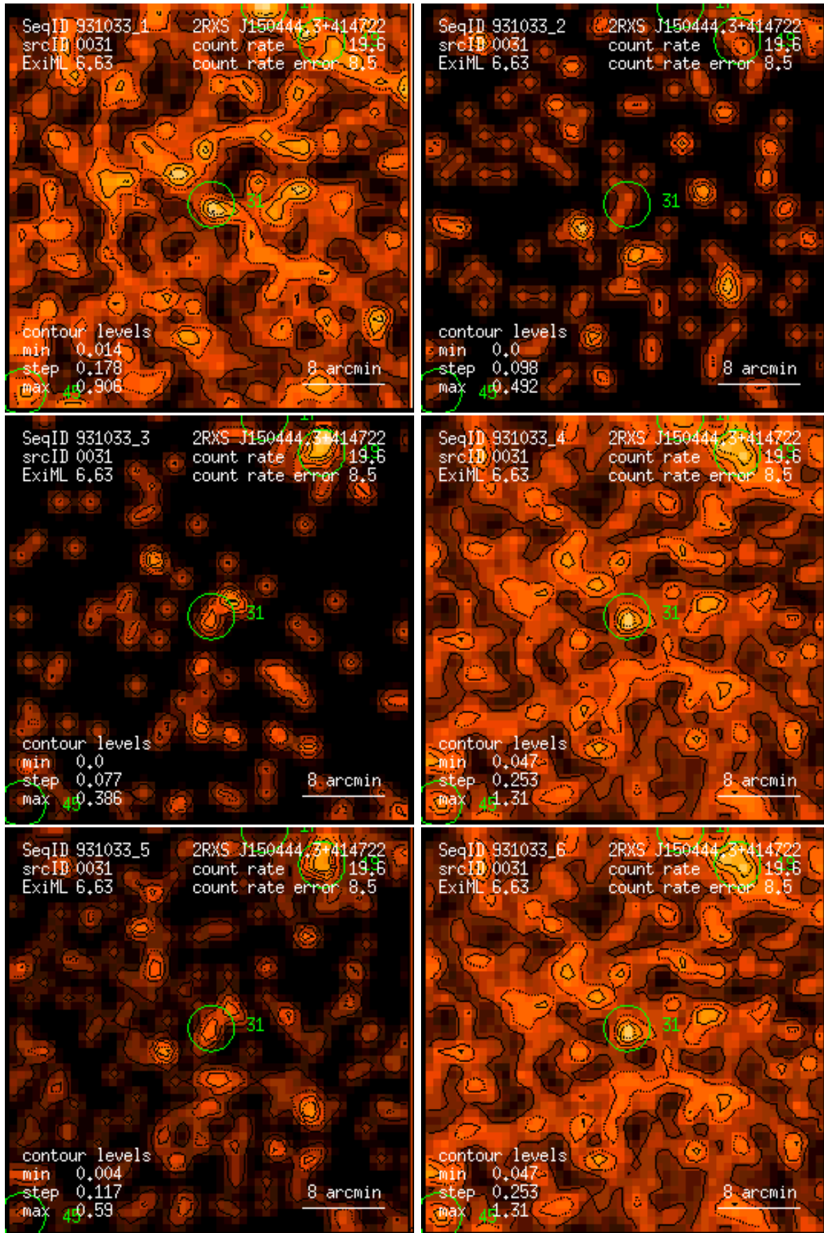
Figure 31: RASS 931033: detection 0031: band rate images, Gaussian filter: (1) PSPC channels 11 – 41, (2) 52 – 90, (3) 91 – 201, (4) 11 – 235, (5) 52 – 201, (6) 11 – 201. Broad band rates in counts/ks. Band rate contour levels in counts/ks/arcmin 2 .
