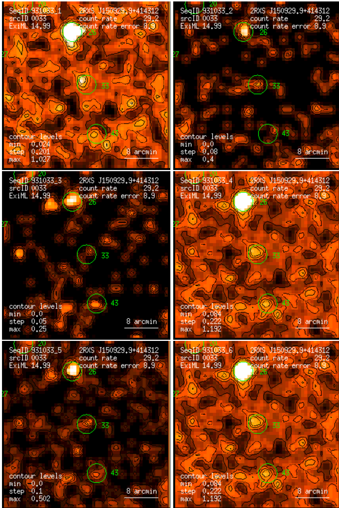
Figure 33: RASS 931033: detection 0033: band rate images, Gaussian filter: (1) PSPC channels 11 – 41, (2) 52 – 90, (3) 91 – 201, (4) 11 – 235, (5) 52 – 201, (6) 11 – 201. Broad band rates in counts/ks. Band rate contour levels in counts/ks/arcmin 2 .
