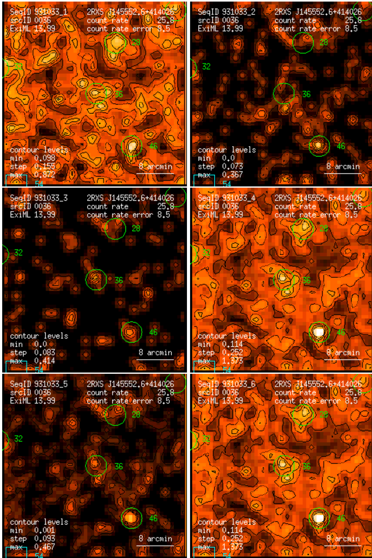
Figure 36: RASS 931033: detection 0036: band rate images, Gaussian filter: (1) PSPC channels 11 – 41, (2) 52 – 90, (3) 91 – 201, (4) 11 – 235, (5) 52 – 201, (6) 11 – 201. Broad band rates in counts/ks. Band rate contour levels in counts/ks/arcmin 2 .
