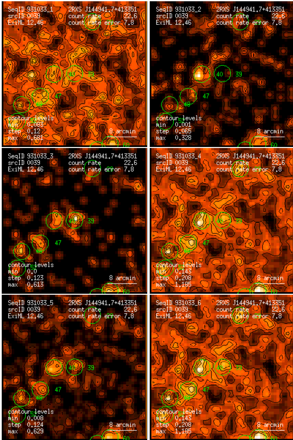
Figure 39: RASS 931033: detection 0039: band rate images, Gaussian filter: (1) PSPC channels 11 – 41, (2) 52 – 90, (3) 91 – 201, (4) 11 – 235, (5) 52 – 201, (6) 11 – 201. Broad band rates in counts/ks. Band rate contour levels in counts/ks/arcmin 2 .
