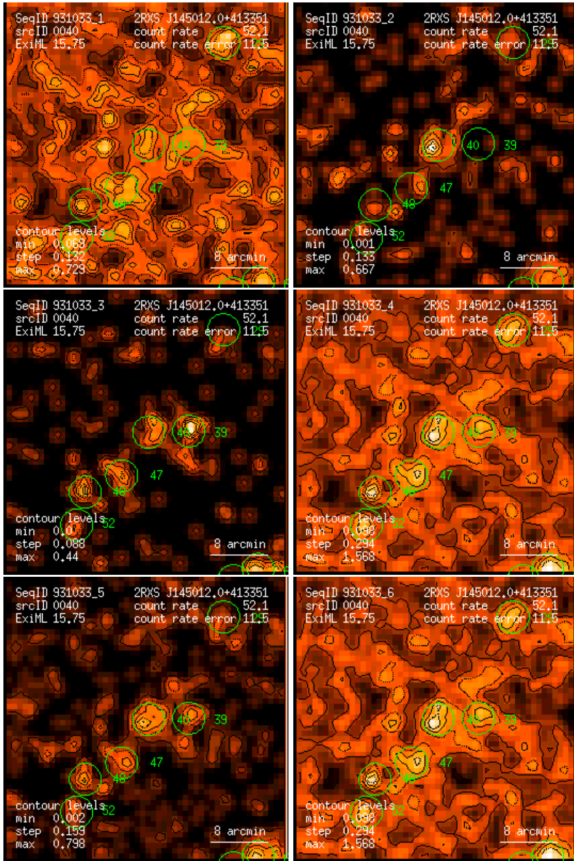
Figure 40: RASS 931033: detection 0040: band rate images, Gaussian filter: (1) PSPC channels 11 – 41, (2) 52 – 90, (3) 91 – 201, (4) 11 – 235, (5) 52 – 201, (6) 11 – 201. Broad band rates in counts/ks. Band rate contour levels in counts/ks/arcmin 2 .
