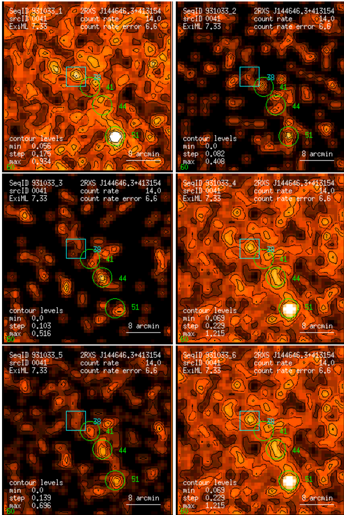
Figure 41: RASS 931033: detection 0041: band rate images, Gaussian filter: (1) PSPC channels 11 – 41, (2) 52 – 90, (3) 91 – 201, (4) 11 – 235, (5) 52 – 201, (6) 11 – 201. Broad band rates in counts/ks. Band rate contour levels in counts/ks/arcmin 2 .
