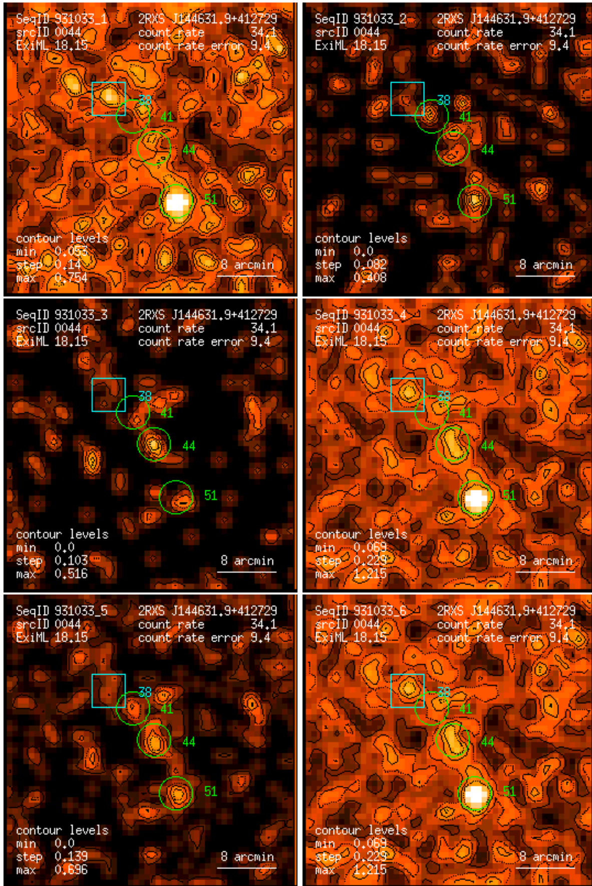
Figure 44: RASS 931033: detection 0044: band rate images, Gaussian filter: (1) PSPC channels 11 – 41, (2) 52 – 90, (3) 91 – 201, (4) 11 – 235, (5) 52 – 201, (6) 11 – 201. Broad band rates in counts/ks. Band rate contour levels in counts/ks/arcmin 2 .
