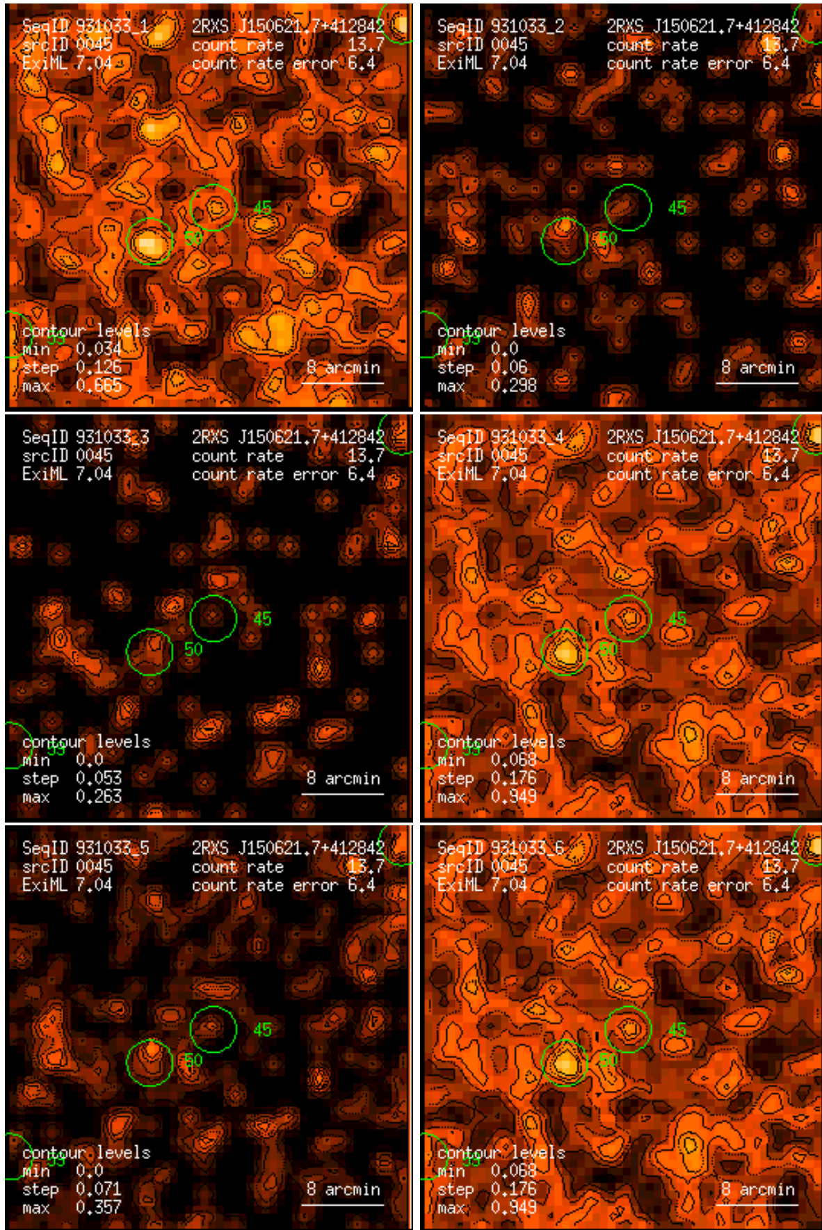
Figure 45: RASS 931033: detection 0045: band rate images, Gaussian filter: (1) PSPC channels 11 – 41, (2) 52 – 90, (3) 91 – 201, (4) 11 – 235, (5) 52 – 201, (6) 11 – 201. Broad band rates in counts/ks. Band rate contour levels in counts/ks/arcmin 2 .
