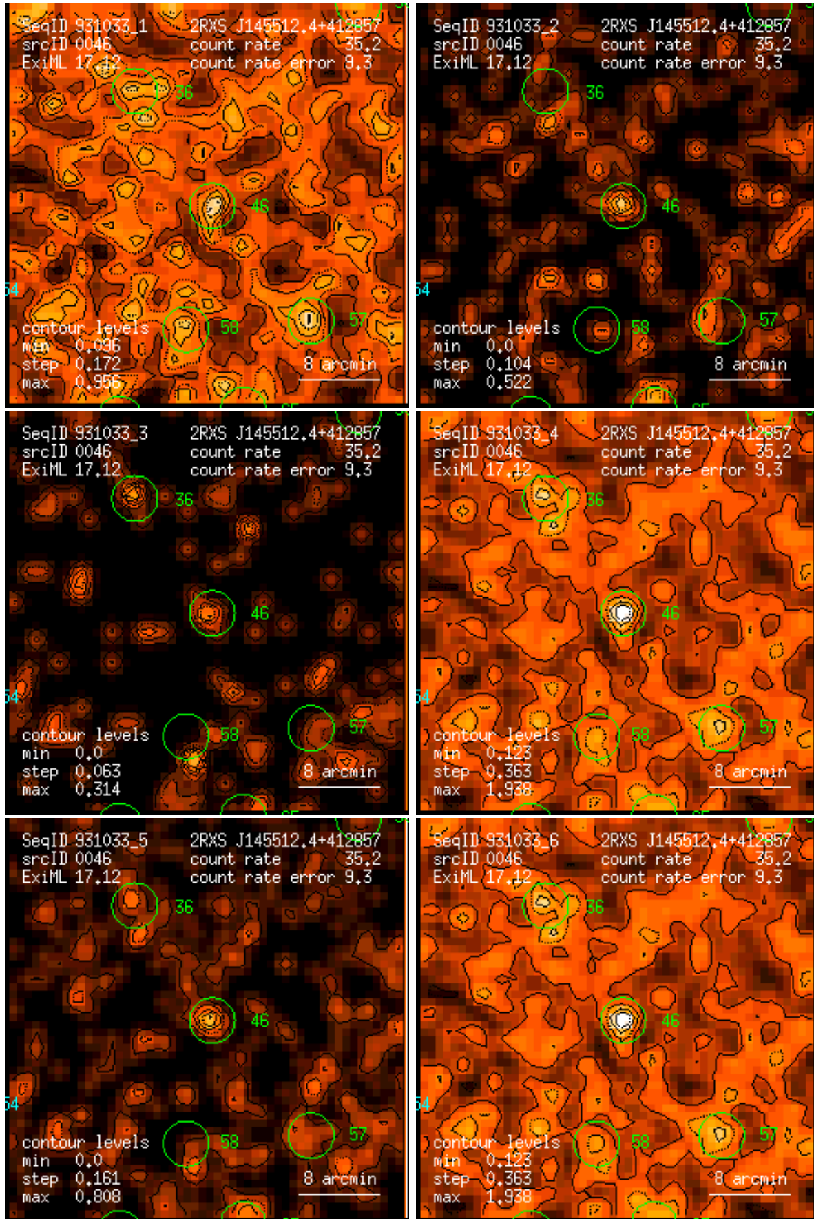
Figure 46: RASS 931033: detection 0046: band rate images, Gaussian filter: (1) PSPC channels 11 – 41, (2) 52 – 90, (3) 91 – 201, (4) 11 – 235, (5) 52 – 201, (6) 11 – 201. Broad band rates in counts/ks. Band rate contour levels in counts/ks/arcmin 2 .
