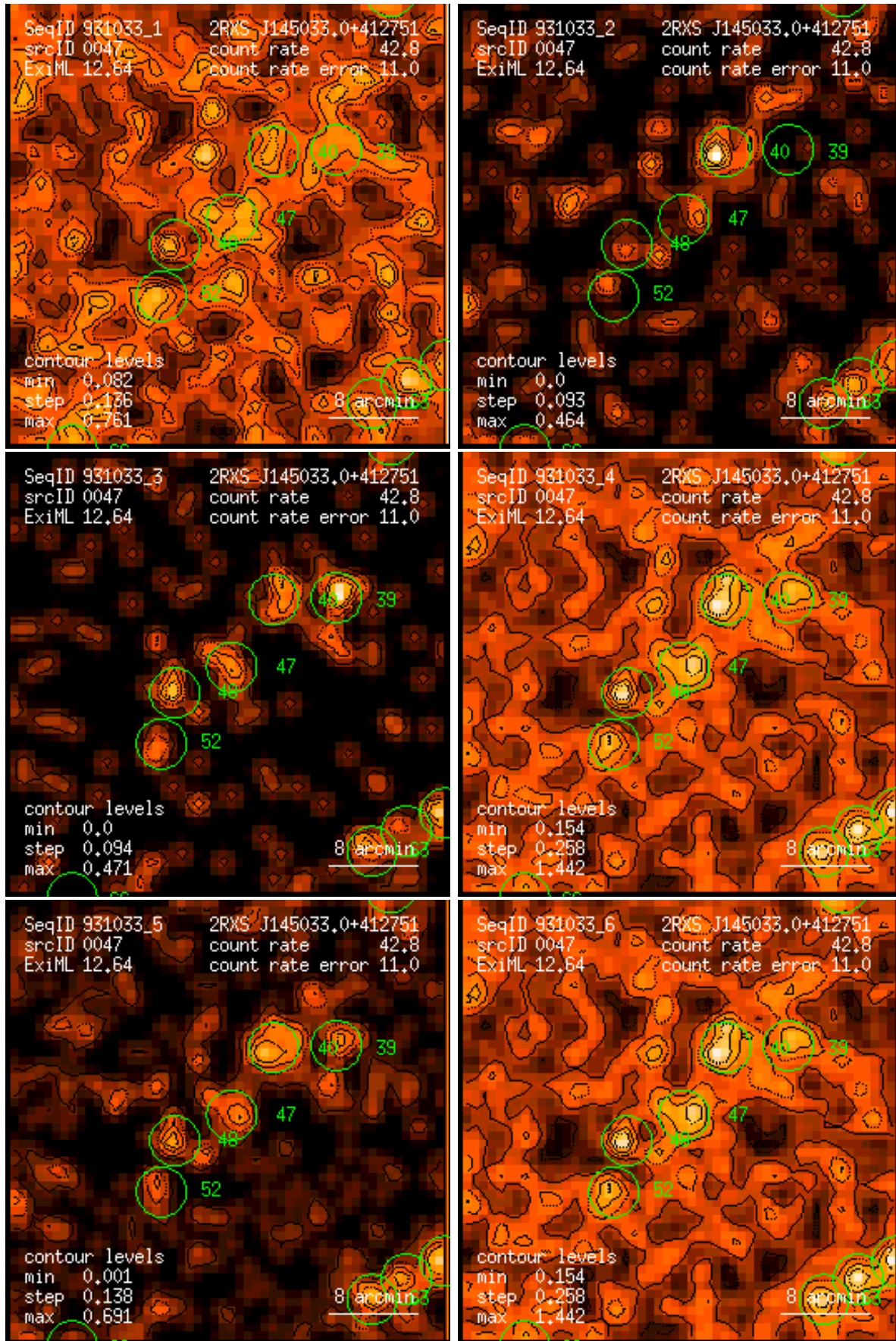
Figure 47: RASS 931033: detection 0047: band rate images, Gaussian filter: (1) PSPC channels 11 – 41, (2) 52 – 90, (3) 91 – 201, (4) 11 – 235, (5) 52 – 201, (6) 11 – 201. Broad band rates in counts/ks. Band rate contour levels in counts/ks/arcmin 2 .
