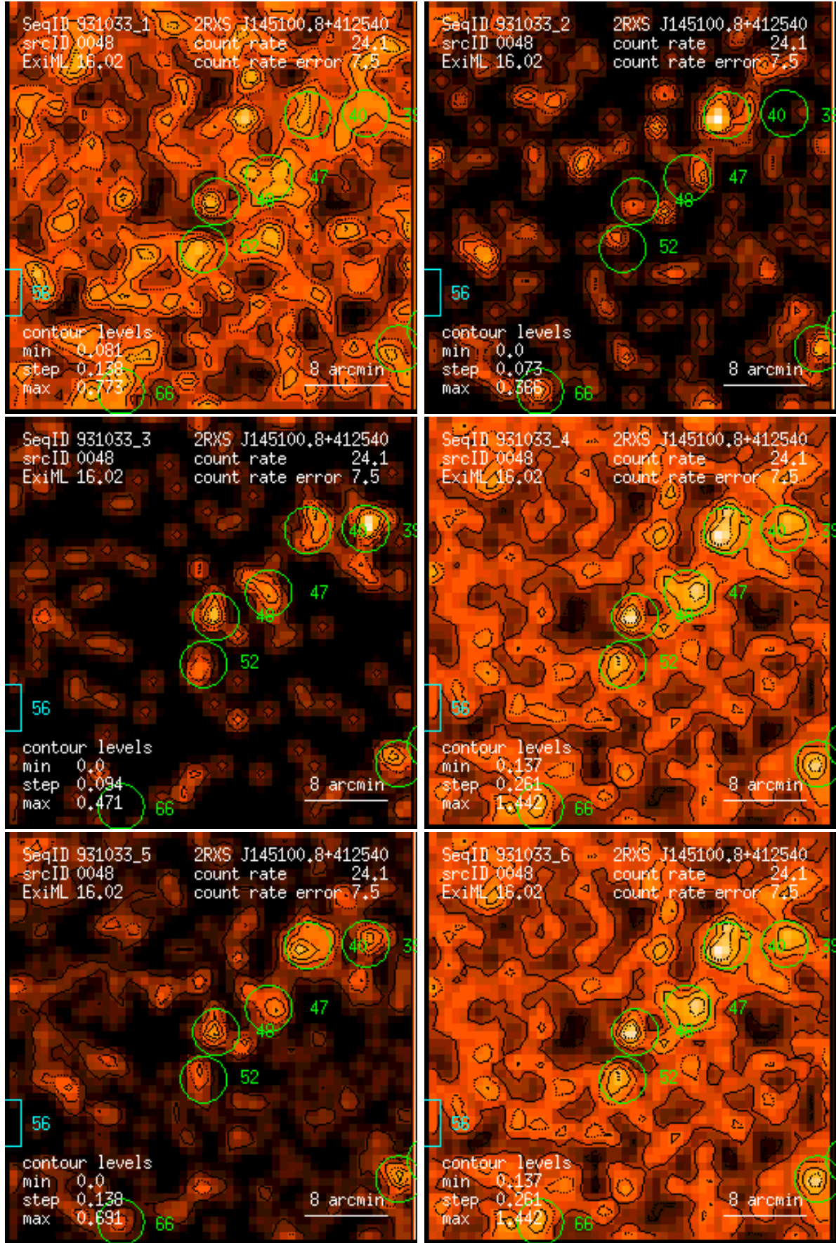
Figure 48: RASS 931033: detection 0048: band rate images, Gaussian filter: (1) PSPC channels 11 – 41, (2) 52 – 90, (3) 91 – 201, (4) 11 – 235, (5) 52 – 201, (6) 11 – 201. Broad band rates in counts/ks. Band rate contour levels in counts/ks/arcmin 2 .
